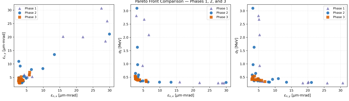
Figure 2: Two-dimensional projections of the physical objective space comparing Phase 1, Phase 2, and Phase 3 Pareto fronts (sourced from pareto.csv ).
