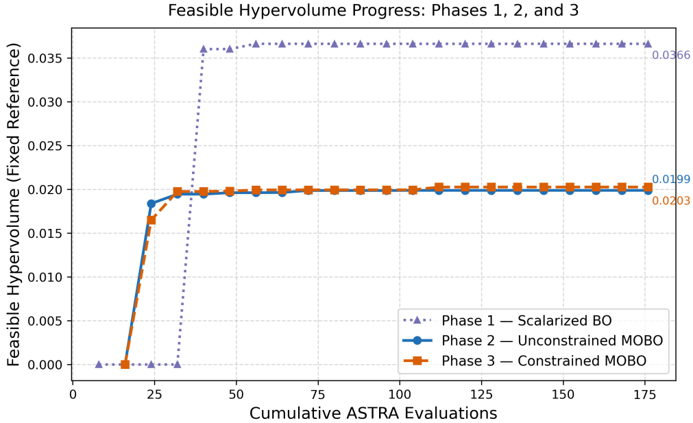
Figure 1: Feasible hypervolume progress over cumulative ASTRA evaluations comparing Phase 1 (Scalarized), Phase 2 (Unconstrained), and Phase 3 (Constrained) MOBO. Final hypervolume values are derived from hypervolume.csv in each campaign run directory.
