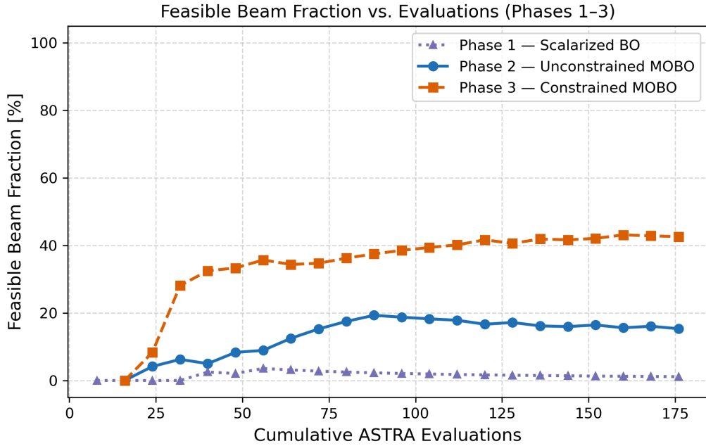
Figure 3: Feasible beam fraction as a function of cumulative ASTRA evaluations comparing Phase 1 (Scalarized), Phase 2 (Unconstrained), and Phase 3 (Constrained) MOBO.
