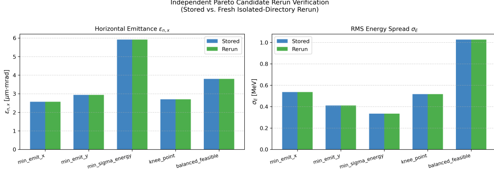
Figure 4: Stored vs. independent rerun objective values for verified Pareto candidates (sourced from verification_summary.csv ). Stored and rerun bars are visually indistinguishable at this scale, confirming exact numerical reproducibility.
