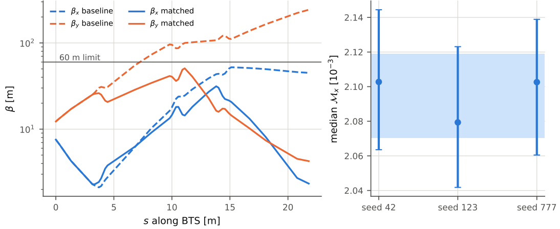
Figure 6. Left: horizontal and vertical \beta functions along the BTS for the baseline (dashed) and matched (solid) quadrupole settings, propagated from the booster extraction optics. Right: median horizontal exit mismatch of three independent 50 000-sample error ensembles with order-statistic 95 % intervals; the band is the pooled interval.
