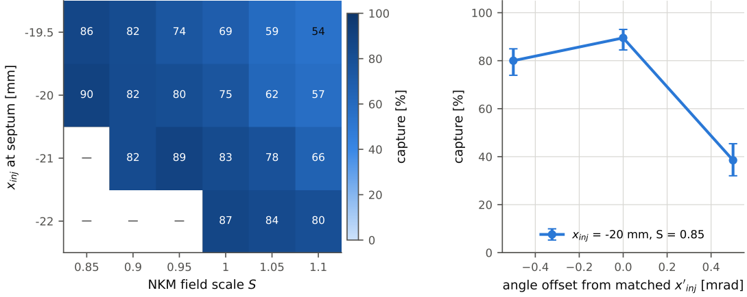
Figure 4. Left: field-map capture (%) at the angle-matched condition versus septum position x_{inj} and field scale S ; dashes mark combinations without an inner matched solution inside the DA. Right: capture versus the angle offset at the selected operating point with 95 % Wilson intervals. Native tracking, 200 particles, 500 turns.
