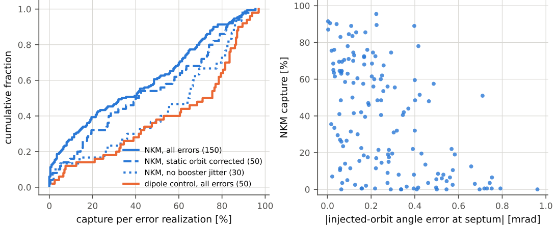
Figure 7. Combined-error robustness at the operating point. Left: cumulative distribution of capture per error realization for the NKM (three seeds), the paired uniform-dipole control and the NKM without booster centroid jitter. Right: NKM capture versus the magnitude of the injected-orbit angle error at the septum exit.
