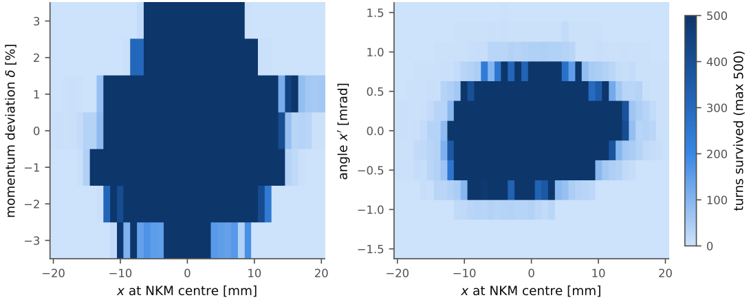
Figure 1. Dynamic aperture at the NKM centre from native element-by-element tracking of single particles for 500 turns (1 mm grid in x ): turns survived versus horizontal position and momentum deviation at x' = 0 (left) and versus horizontal position and angle at \delta = 0 (right).
