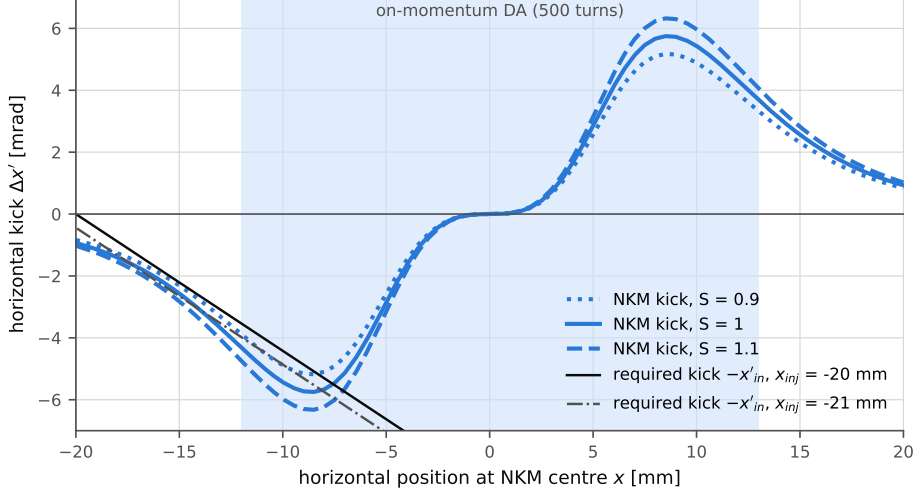
Figure 2. Horizontal NKM kick at y = 0 for field scales S = 0.9, 1.0 and 1.1 (blue), compared with the kick required to cancel the incoming angle of a beam launched from the septum at x_{inj} = -20 and -21 mm with angle x'_{in} = (x - x_{inj})/L , L = 2.26 m (black). Intersections are angle-matched operating points. The shaded band is the on-momentum dynamic aperture.
