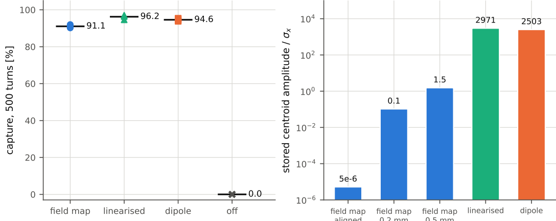
Figure 5. Paired comparison at the operating point. Left: capture of four independent 500-particle bunches (markers) and their mean (bar) for each kick model. Right: stored-beam centroid amplitude in units of the rms beam size after one passage for the NKM aligned and offset by 0.2 and 0.5 mm from the stored orbit, and for the calibrated controls (logarithmic scale).
