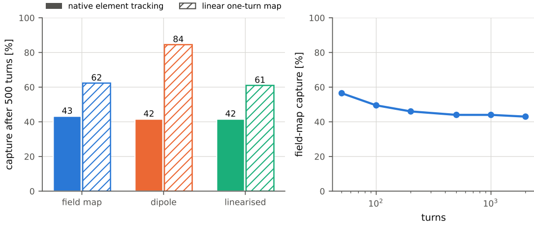
Figure 3. Left: capture after 500 turns at the provisional point for native element tracking (filled) and the linear one-turn map (hatched) on identical 200-particle bunches (field map: mean of three bunches). Right: field-map capture versus the number of turns (native tracking).
