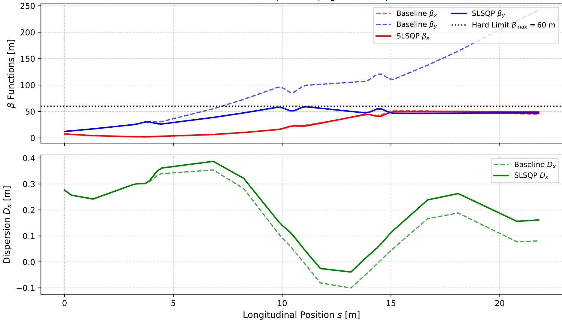
BTS Transfer Line Optics Propagation Comparison
