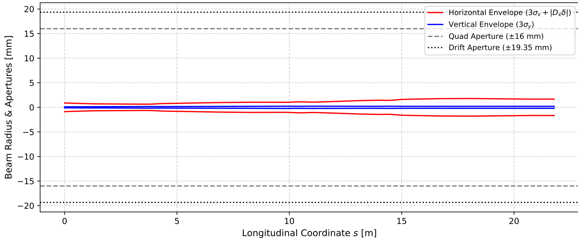
Transverse 3\sigma Beam Envelopes Along BTS Line
