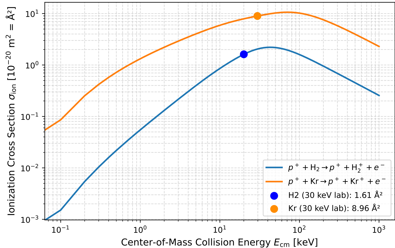
Proton-Impact Ionization Cross Sections ( \text{H}_2 vs Kr)
