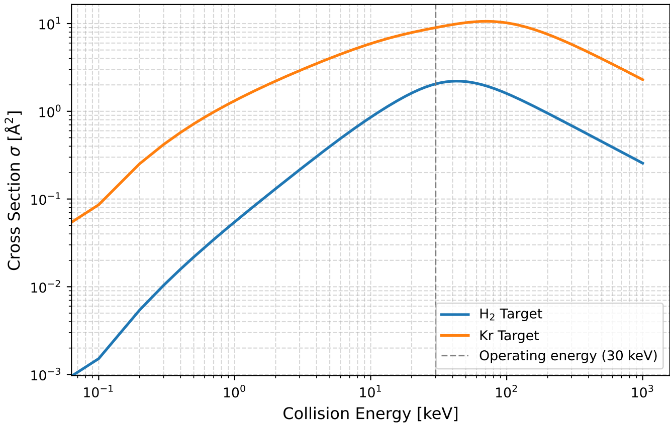
Proton-Impact Ionization Cross Sections \sigma(E)
