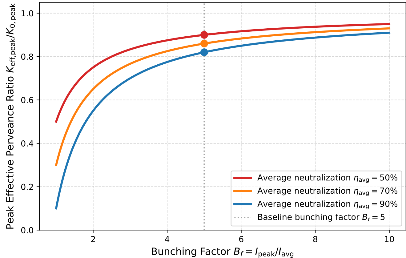
RF-Bunched Beam Peak Space-Charge Reduction
