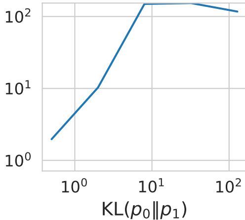
Density Ratio Error on Test Data
