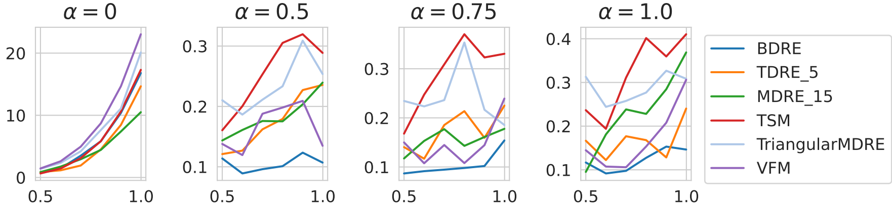
ELBO Estimation Error
