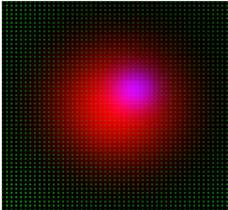
TriangularMDRE (MAE: 35.355)
