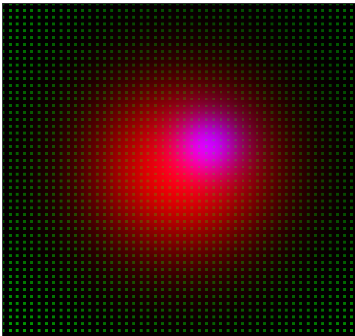
TriangularMDRE (MAE: 35.355)
