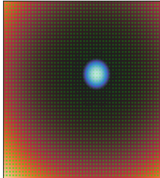
MDRE_15 (MAE: 29.855)
