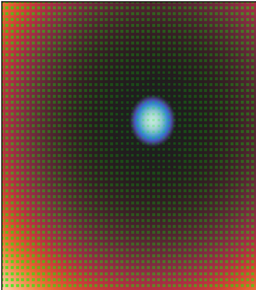
TriangularMDRE (MAE: 35.355)
