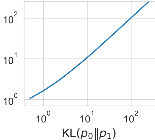
Density Ratio Error on Test Data
