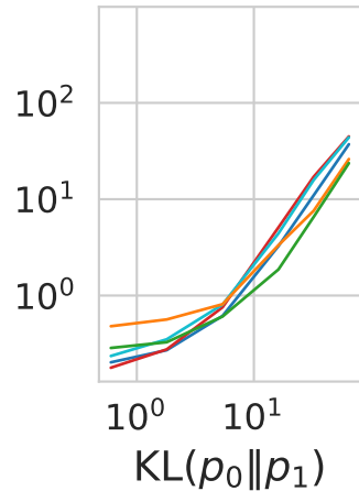
Median Absolute Error (Test Set)
