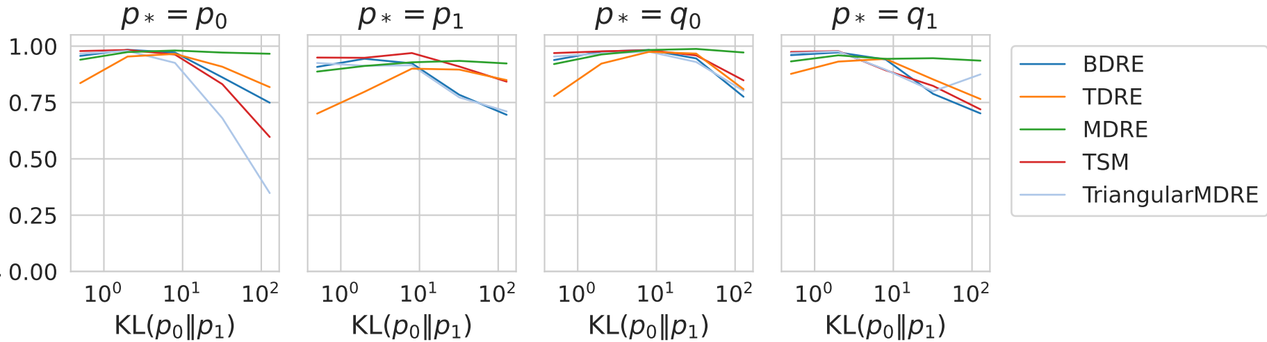
Spearman Correlation
