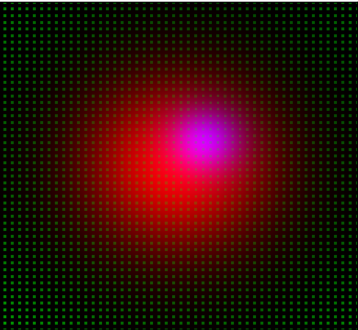
MDRE_15 (MAE: 29.855)
