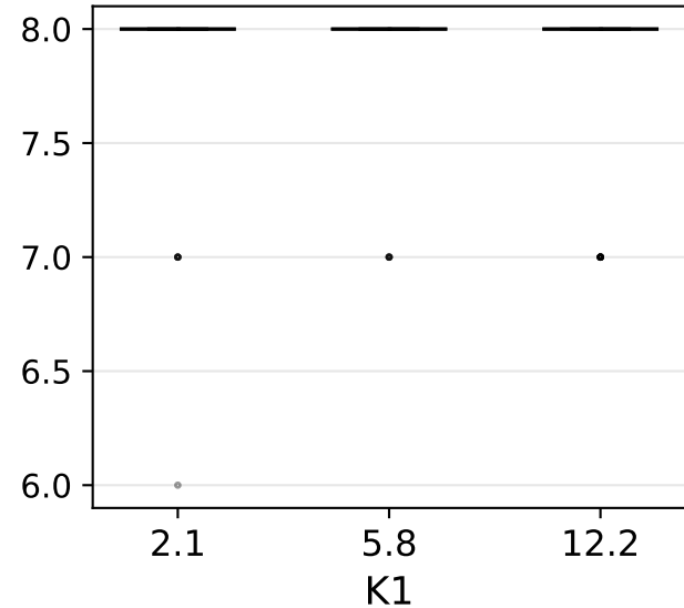
gmm_modes
