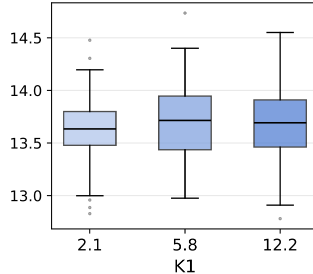
twonn_id
