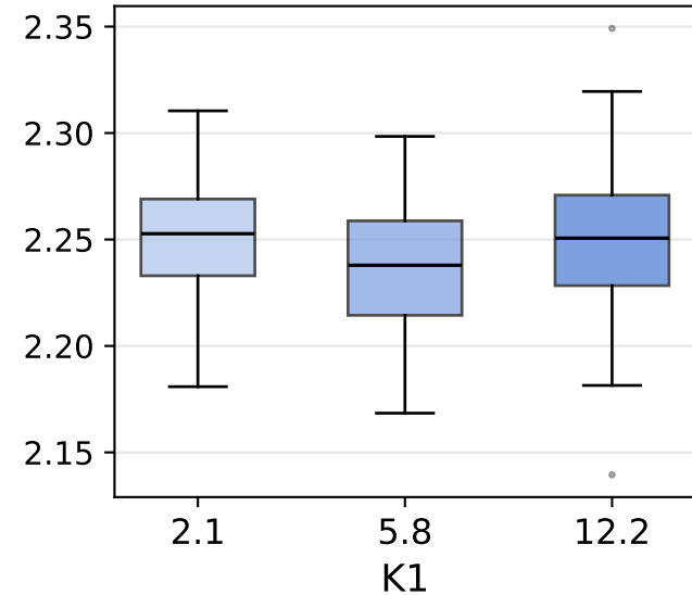
part_ratio
