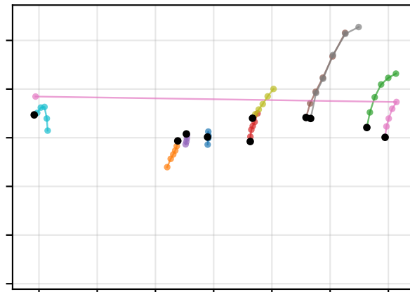
p_* seed=0
