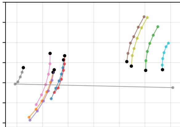
p_* seed=0
