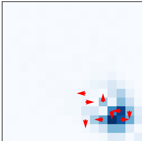
p_0(d_O) seed=1
