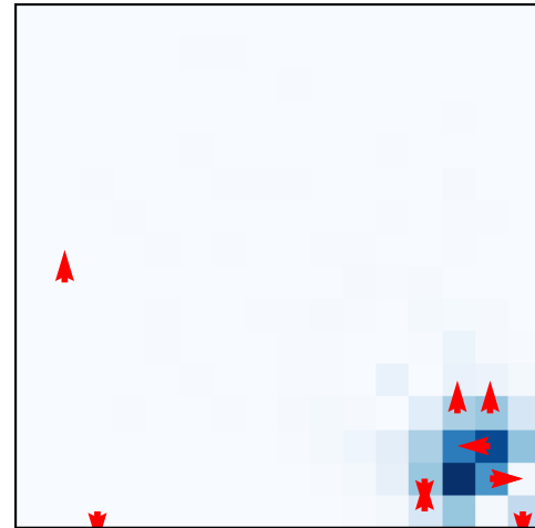
p_* seed=1
