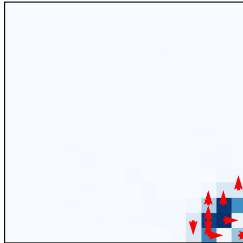
p_1(d_E) seed=1
