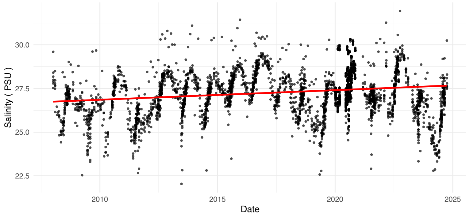
Salinity from 2008–2024
