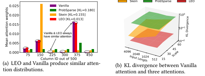
Figure 2: Illustration of attention distribution with attention weights (left) and KL divergence (right) between Vanilla cross-modal attention [49] and the other three attention distributions — the lower the closer to Vanilla attention. Scale is the constant factor independent of input length.
