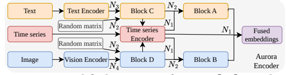
Figure 8: Simplified structure of Aurora [54] encoder.
