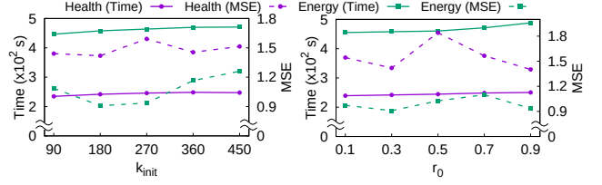
Figure 12: Parameter sensitivity varying k_{init} and r_0 .
