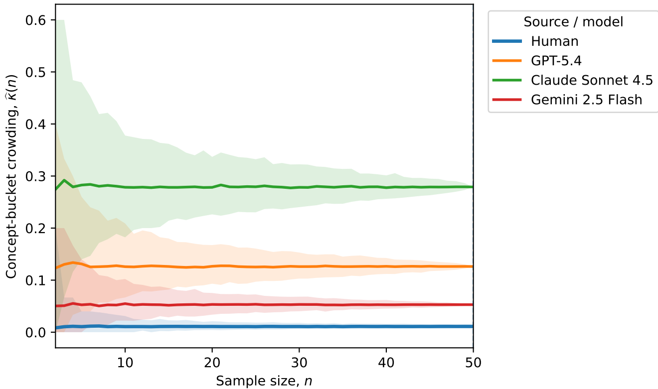
AUT concept-bucket rarefaction
