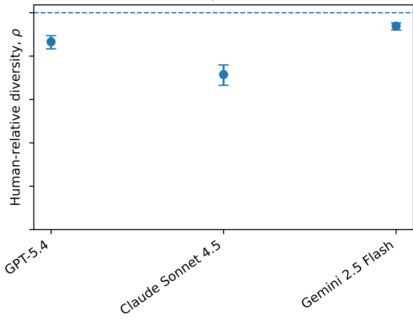
Concept Bucket
