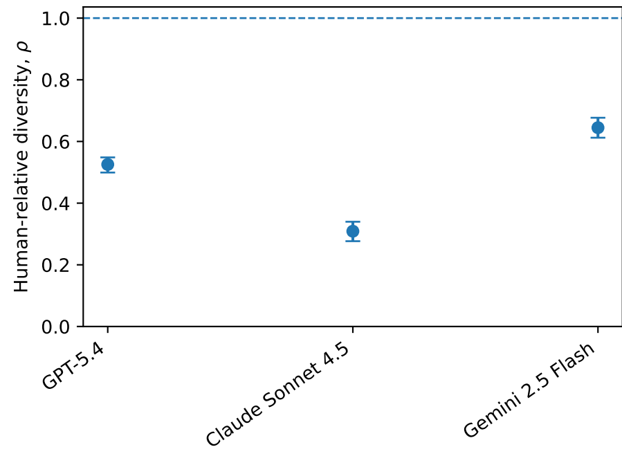
Semantic
