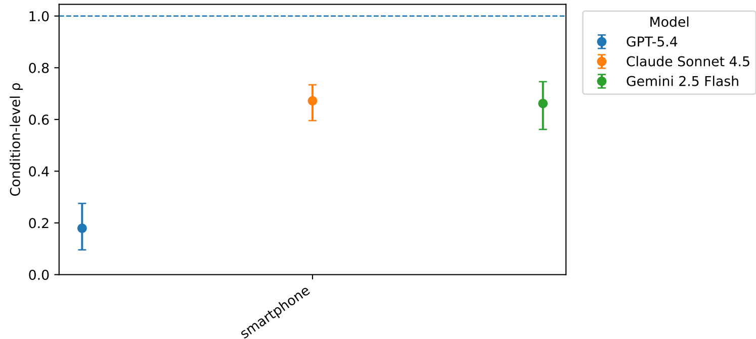
Condition-level human-relative diversity: SLOGAN
