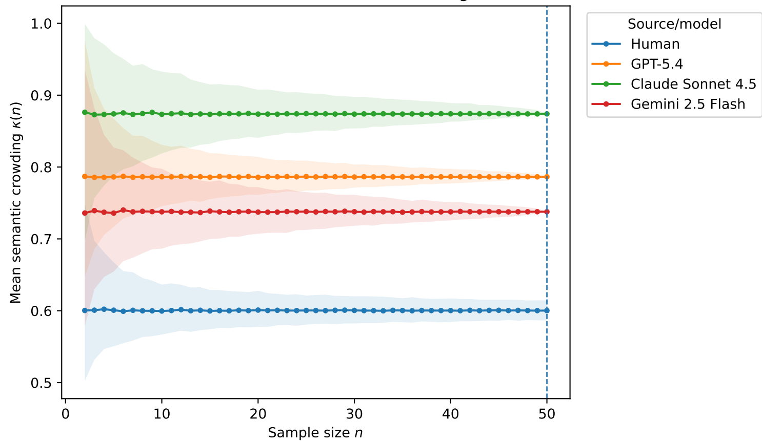
Task-level saturation of semantic crowding: AUT
