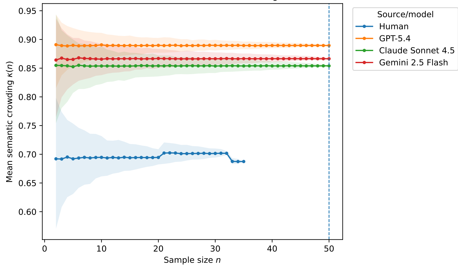
Task-level saturation of semantic crowding: STORY
