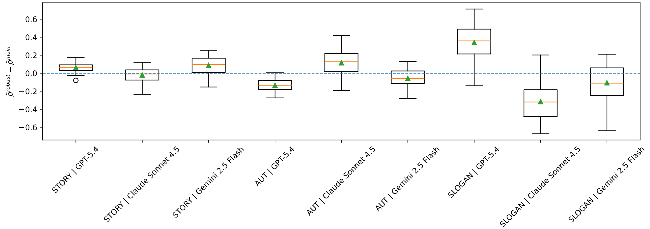
Persona robustness shifts relative to main neutral estimate
