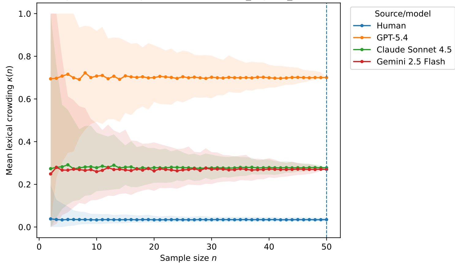
Slogan lexical-template saturation: char_trigram_jaccard
