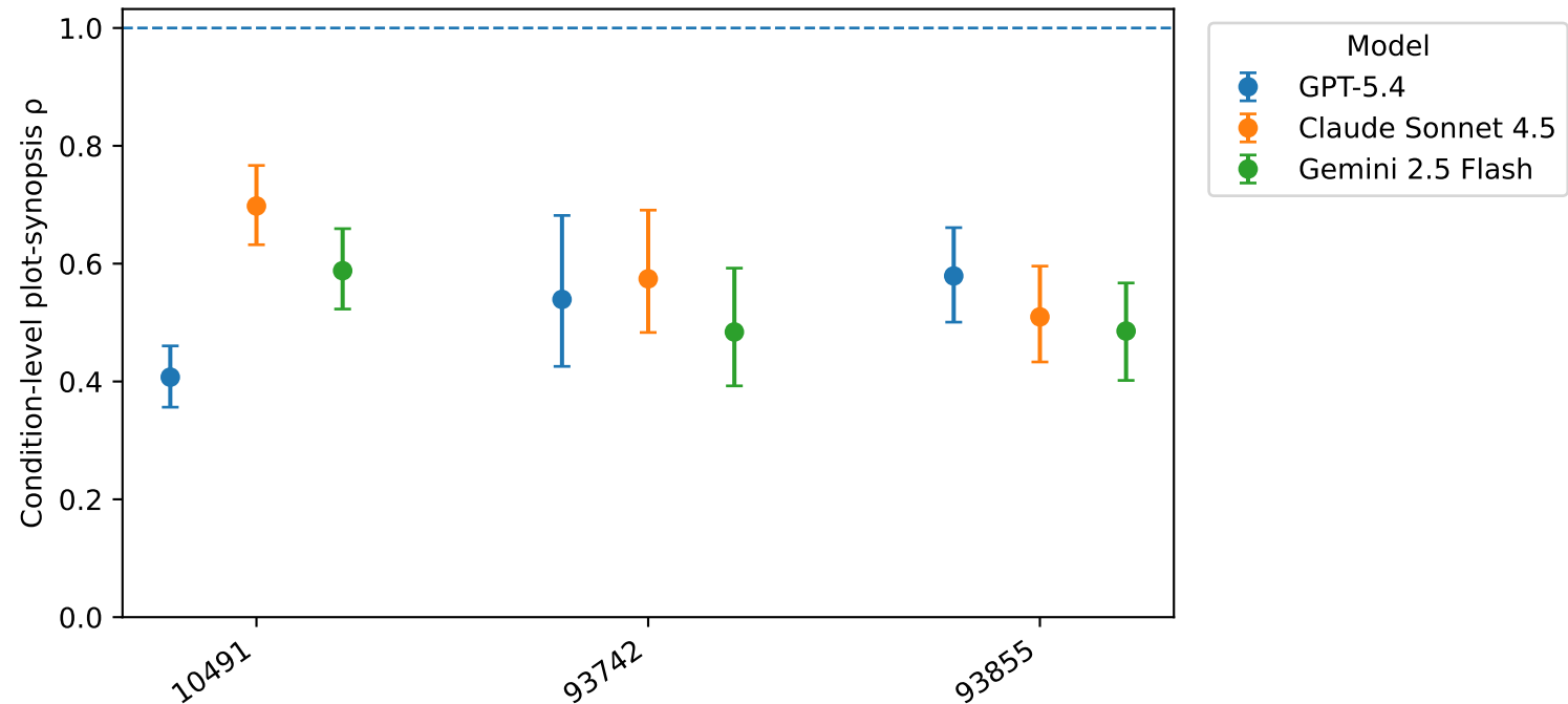
Story plot-synopsis crowding by prompt
