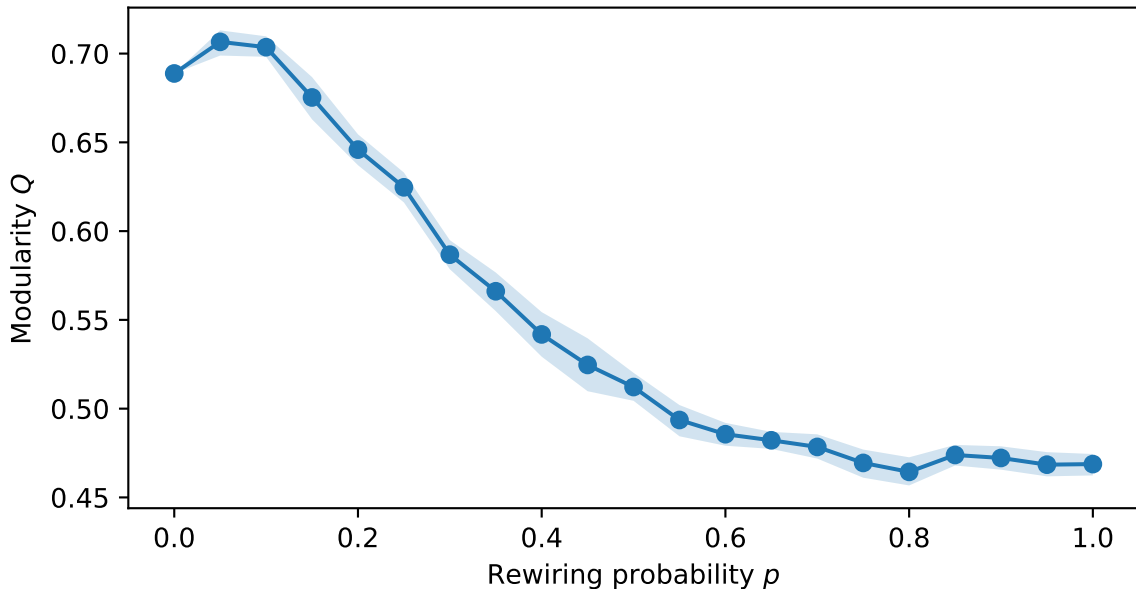
Semantic modularity decreases with WS rewiring
