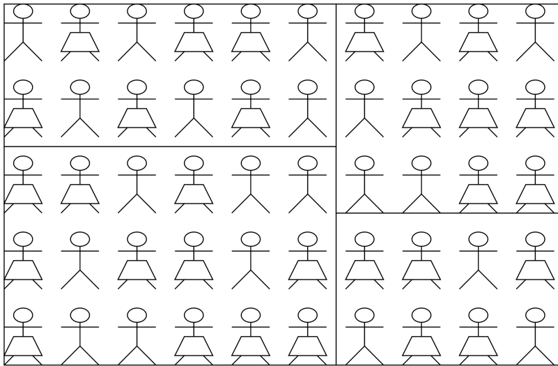
Figure 4: Cluster sampling
