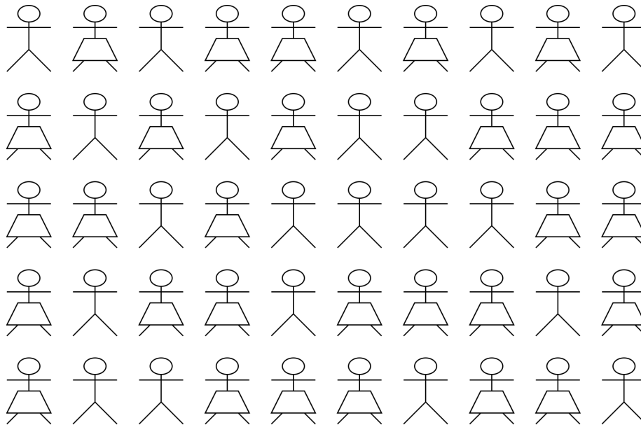
Figure 1: convenience sample
