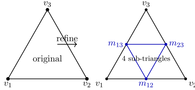
Figure 20.2: 1-to-4 triangle refinement: each edge is split at its midpoint, producing four congruent sub-triangles.
