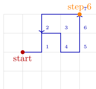
Figure 27.2: Random walk on a grid: at each step, move to a uniformly random neighboring vertex.
