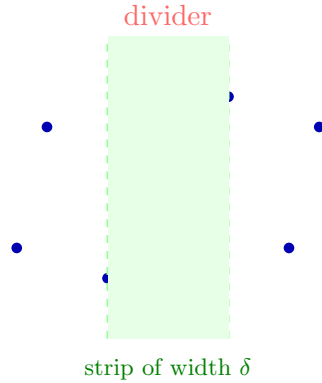
Figure 13.1: Closest pair: divide-and-conquer splits points along a vertical line. The closest pair may cross the dividing strip.
