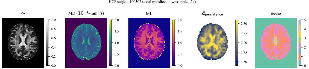
Figure 7. Axial midslice maps in a representative HCP-YA subject (downsampled 2 \times in-plane for tractability of the voxelwise persistence step). From left to right: FA, MD, mean kurtosis MK, \hat{\alpha}_{\text{persistence}} , and the derived tissue mask (WM, GM, CSF, midsagittal corpus callosum). The persistence-tail map captures the same broad white-vs-grey contrast as the kurtosis map while emphasising compact tract structure.
