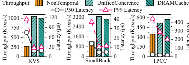
Figure 12. Effectiveness of unified cache coherence.
