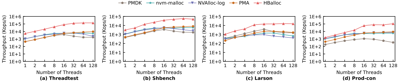
Fig. 15. Throughputs on a single socket configuration.
