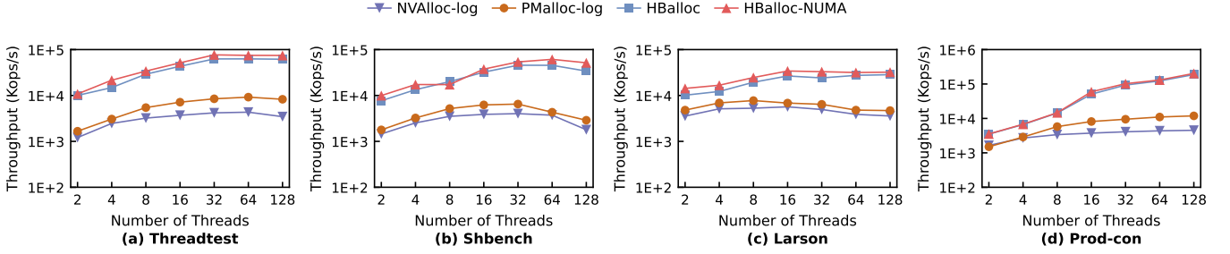
Fig. 14. Throughputs on the dual-socket configuration with NUMA effects.
