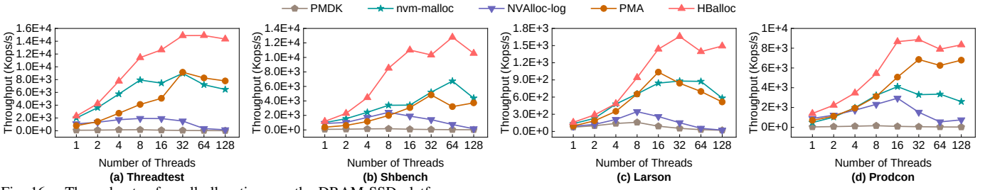
Fig. 16. Throughputs of small allocations on the DRAM-SSD platform.
