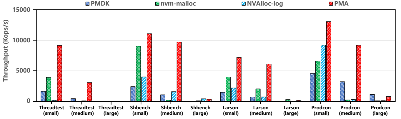
Fig. 2. The throughputs of existing PM allocators for various benchmarks.
