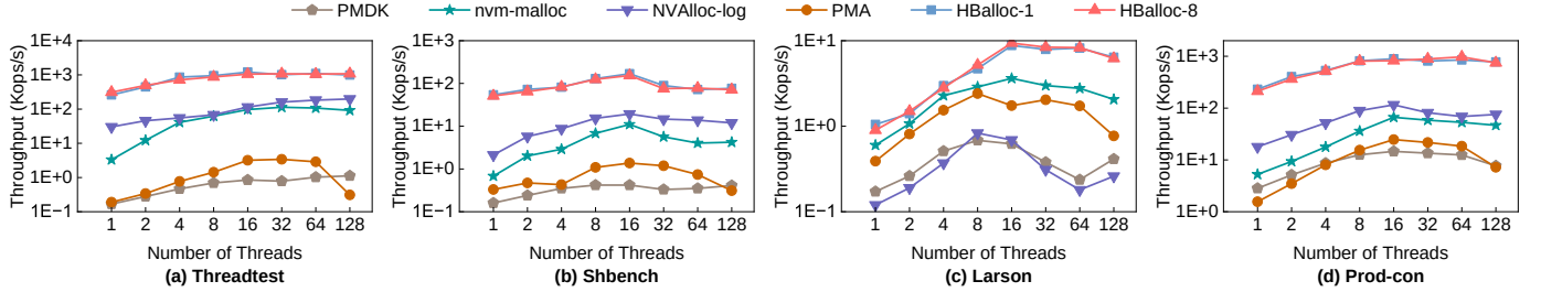
Fig. 8. Throughputs (log10 scaled) of large allocations across different PM allocators.
