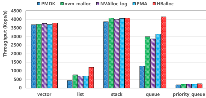
Fig. 13. The throughputs of persistent data structures with different PM allocators.
