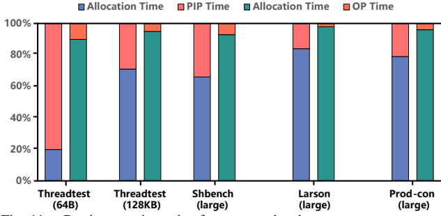
Fig. 11. Persistent pointer dereference overheads.
