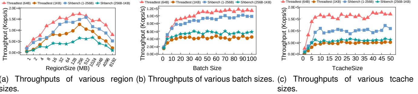
Fig. 10. The throughputs of HBalloc under different region sizes, batch sizes and tcache sizes.
