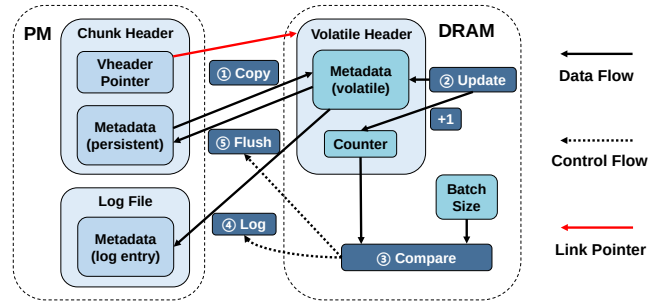
Fig. 5. The key data structure and workflow of the batched persistence mechanism.
