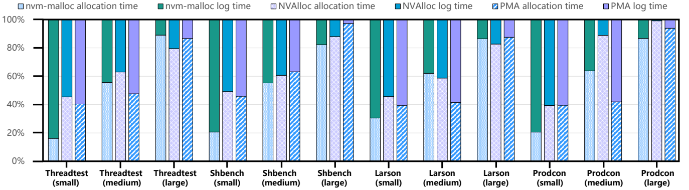
Fig. 3. The log overhead ratios of existing PM allocators for various benchmarks.
