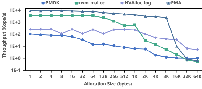
Fig. 1. The throughputs of existing PM allocators for various allocation sizes.
