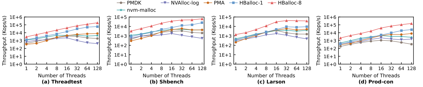
Fig. 7. Throughputs (log10 scaled) of small allocations across different PM allocators.
