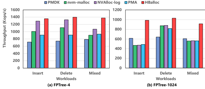
Fig. 12. The throughputs of FPTree with different PM allocators.
