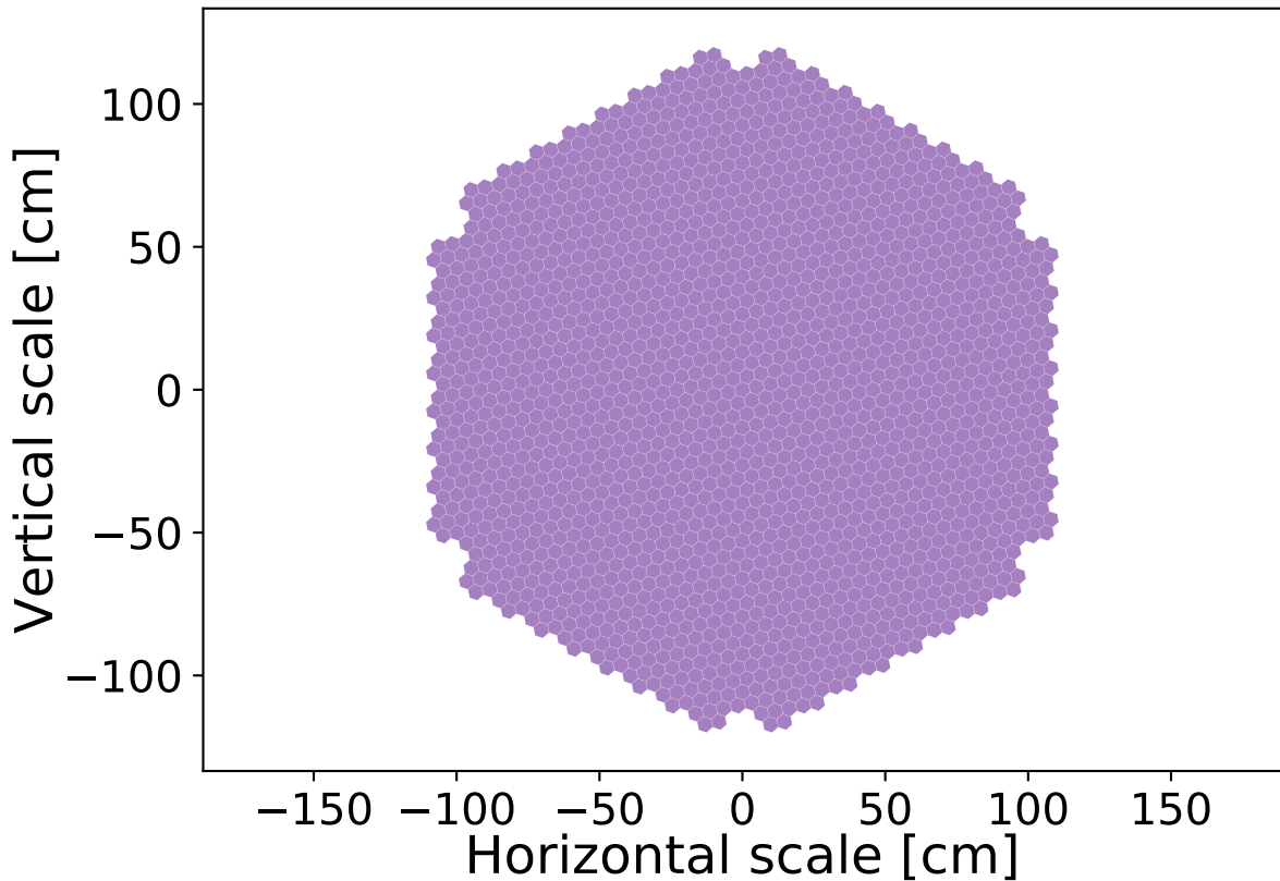
Pixels layout in LST camera
