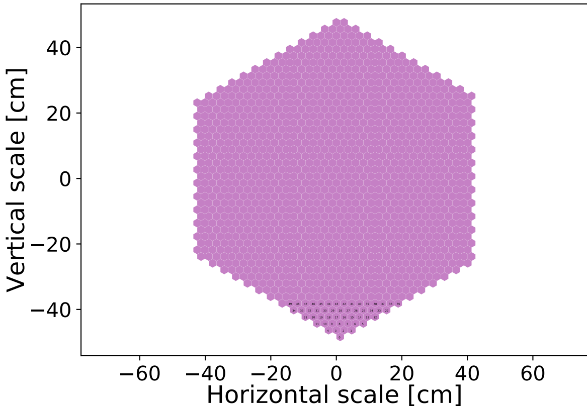
Pixels layout in SST 1M camera
