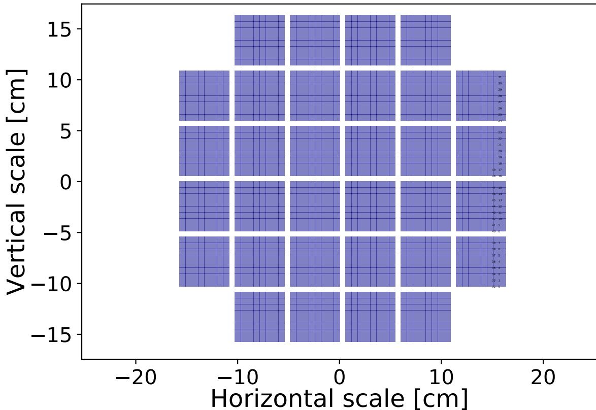
Pixels layout in SST-2M GCT-M camera
