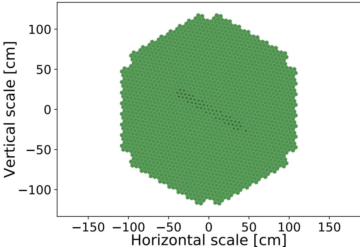
Pixels layout in MST NectarCam camera
