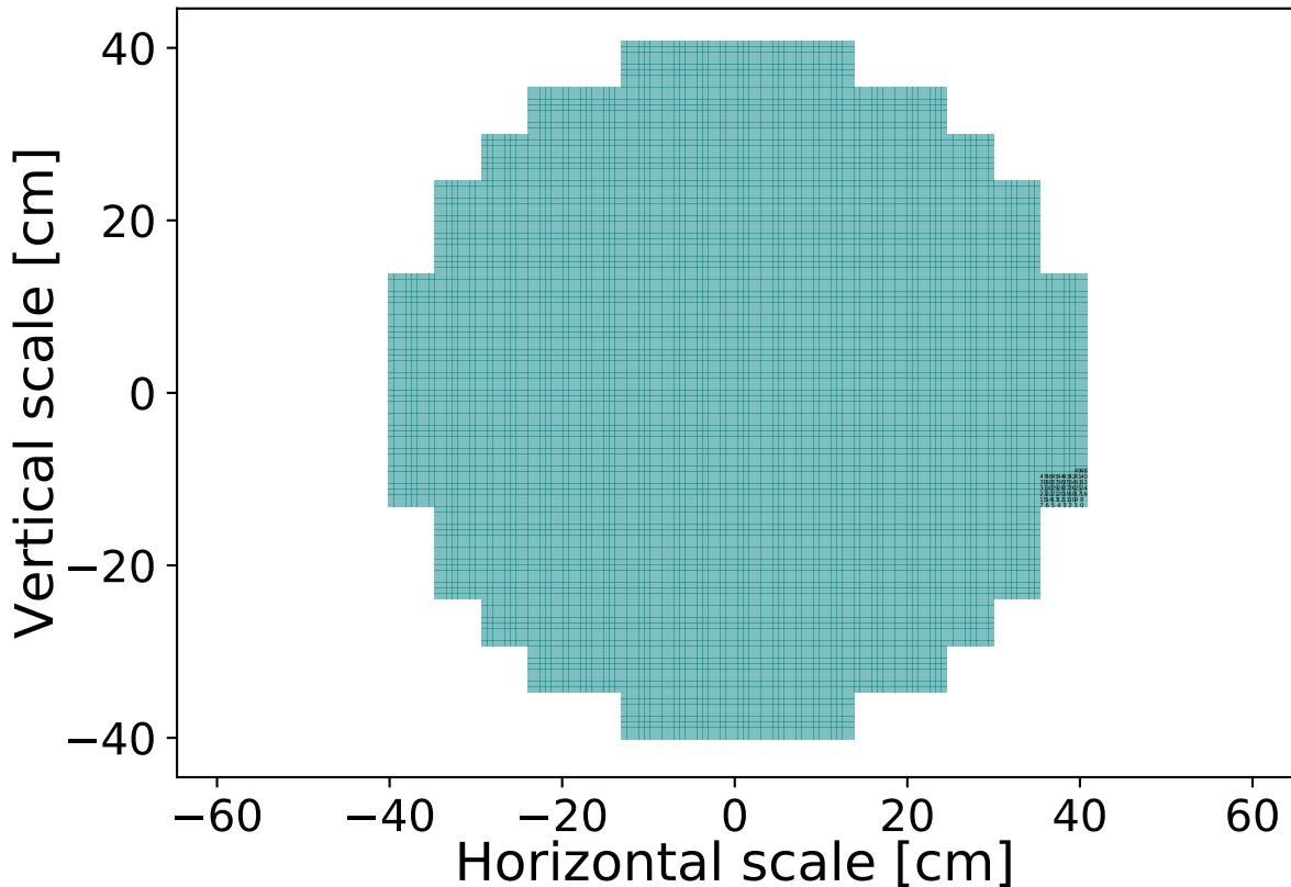
Pixels layout in SCT camera
