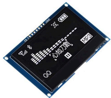
HiLetgo 2.42" SSD1309 128x64 OLED Display Module 2.42 Inch OLED LCD Display Module ...
