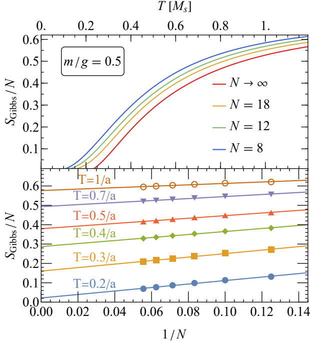
FIG. 12. Top panel: Gibbs entropy density for different values of the system size N as a function of temperature obtained with exact diagonalization as explained in the main text. Bottom panel: linear extrapolation in 1/N of the Gibbs entropy density for several values of the temperature. The intercepts with the y axis correspond to the infinite volume extrapolation and are used in the top panel. Fermion coupling and mass are g = 0.5/a, m = 0.25/a .
