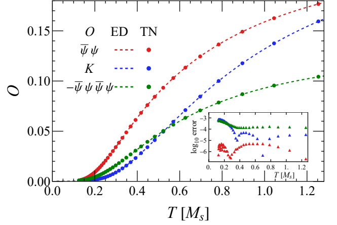
FIG. 14. Local observables (chiral condensate \bar{\psi}\psi , kinetic energy density K and condensate-condensate correlation function \bar{\psi}\psi\bar{\psi}\psi ) obtained with exact diagonalization (ED) and the purification algorithm realized with tensor network methods (TN) shown as a function of temperature. Inset: logarithm of the absolute value of the difference between ED and TN.
