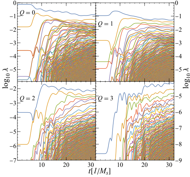
FIG. 6. Entanglement spectrum in four different charge sectors for a subsystem of size L = 12 as a function of time, shown as the logarithm for legibility. Total size of the system is N = 100 , fermion coupling and mass are g = 0.5/a, m = 0.5g .
