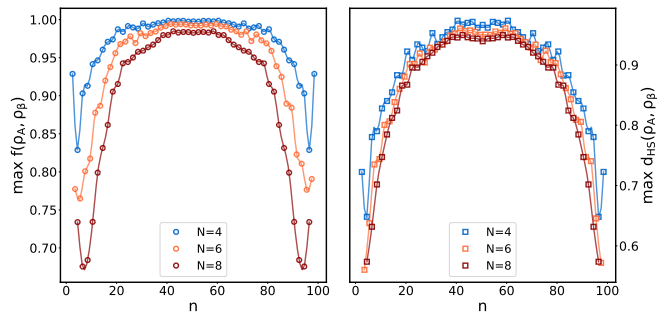
FIG. 9. Spatial cut at time t \approx 40/M_s . We move a subinterval of size N = 4, 6, 8 through the system. The x -axis indicates the center site of the subinterval. The left figure displays the maximal normalized overlap with the thermal states (obtained for N = 12 ). The right plot shows the complement of the minimal HS distance.
