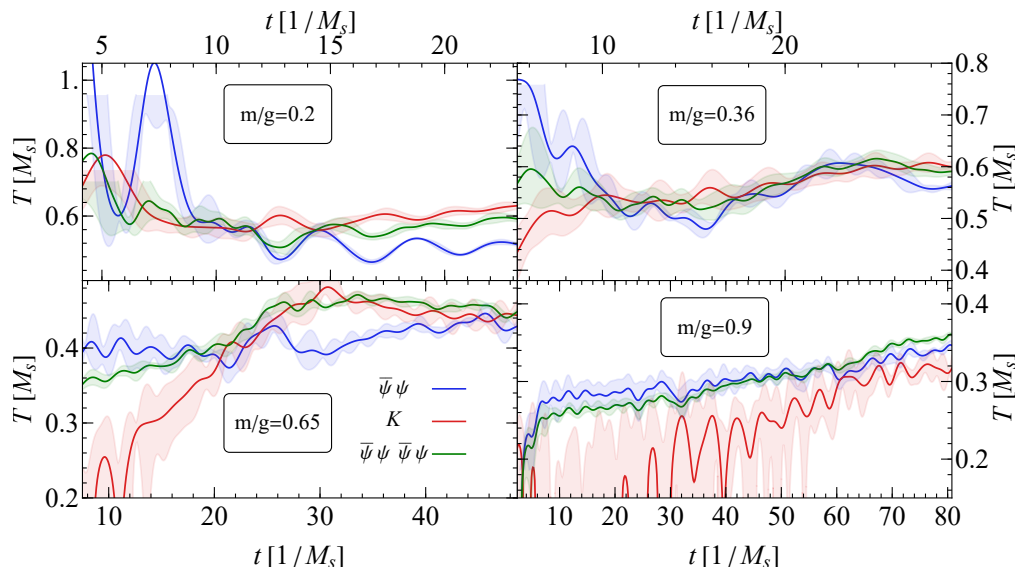
FIG. 4. Comparison of the dynamics of thermalization in the jet simulation from local observables at several values of fermion mass m . Temperature and time are expressed in the physical units, namely the pseudoscalar meson mass, as explained in the text. Fermion coupling is g = 0.5/a in all cases. Thermalization at large fermion mass, m/g = 0.9 , is slower compared to m/g \sim 0.5 . For small fermion mass, m/g = 0.2 , due to computational cost we could not go to comparable physical times, however in the available time interval the observables equilibrate to slightly different effective temperatures, indicating a lesser degree of thermalization compared to m/g \sim 0.5 .
