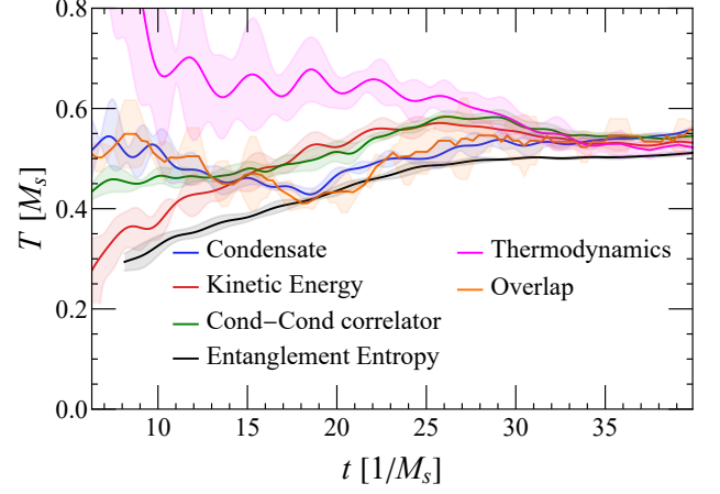
FIG. 3. Effective temperatures in the jet simulation found from the local observables, entanglement entropy, thermodynamic relation (24) and maximizing the overlap between the jet reduced density matrix and a thermal density matrix. The procedure to evaluate temperature from the chiral condensate, kinetic energy and condensate-condensate correlator is described in Sec. III. Extraction of the effective temperature from the entanglement entropy and the thermodynamic relation (24) are described in Sec. IV. Finding the temperature by overlapping density matrices is discussed in Section V. Fermion coupling and mass are g = 0.5/a , m = 0.5g . Units of temperature and time are derived from the meson mass M_s corresponding to the energy of the first excited state in the infinite volume limit (see Appendix C for details).
