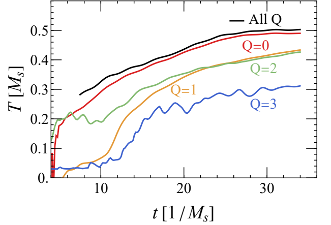
FIG. 19. Effective temperature extracted from the time evolution of symmetry-resolved entanglement entropy in different charge sectors. Infinite volume extrapolated Gibbs entropy is used to extract the temperature. Black line corresponds to the full entanglement entropy and is the same as the black line in Fig. 3. Q = 0 symmetry-resolved temperature turns out to be very close to the full entropy temperature, while in the charged sectors the effective temperature is lower.
