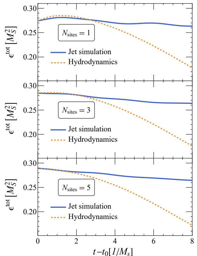
FIG. 11. Energy density as a function of time for the central physical region corresponding to N_{\text{sites}} = 1, 3 and 5 sites. Solid blue lines correspond to the jet simulation results, dashed orange lines are the results from FluiduM.
