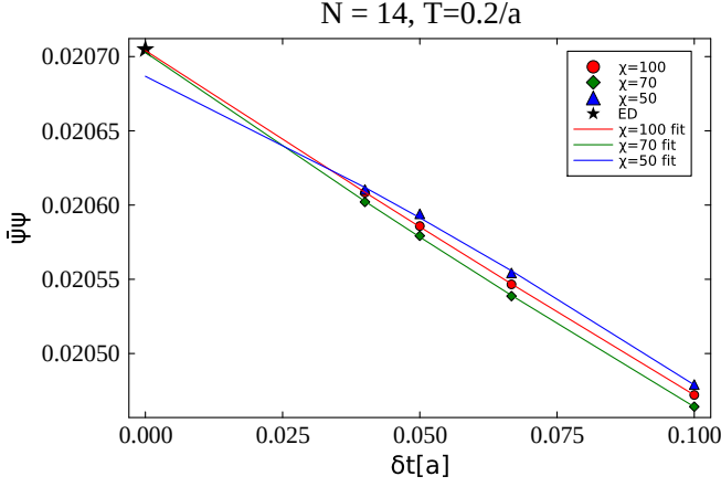
FIG. 13. Comparing purification to exact diagonalization (ED) using chiral condensate \bar{\psi}\psi (with the vacuum value subtracted) as an observable. Purification results for various fixed bond dimension values \chi are shown against the imaginary time evolution timestep \delta t . Quadratic fits in \delta t are performed to extrapolate to \delta t \rightarrow 0 . The extrapolation greatly improves the agreement with the exact result. Simulations with the bond dimension larger than 100 coincide with the one as 100, so at \chi = 100 the MPS truncation error is already negligible.
