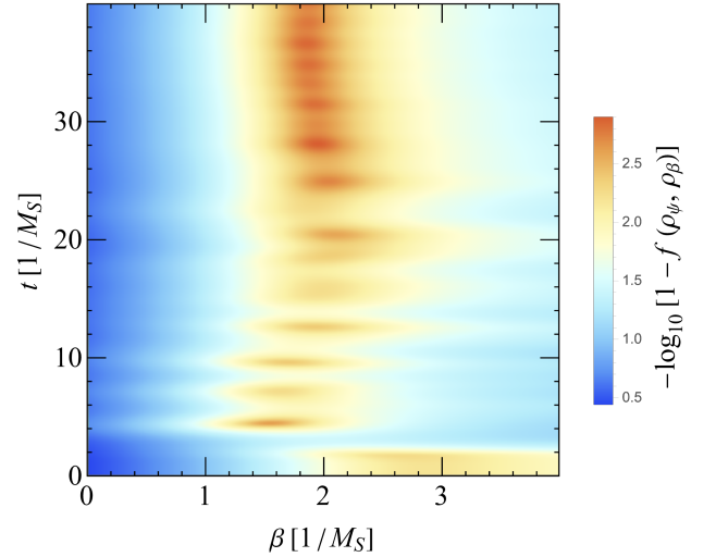
FIG. 20. Overlap of a reduced density matrix obtained from the jet system state |\Psi(t)\rangle for a subsystem with L = 2 (namely, the subsystem consisting of sites number 49 and 50) with a thermal state \rho_\beta as function of t and \beta , shown as a logarithm of deviation from 1 for visual clarity.
