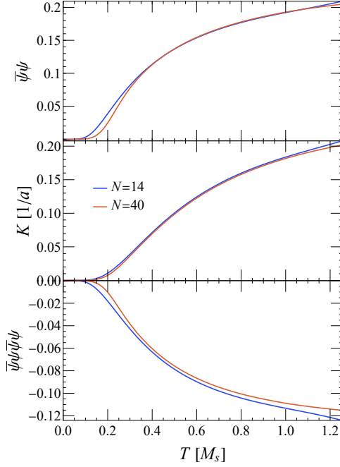
FIG. 15. Average values of local observables (top panel: chiral condensate, middle panel: kinetic energy, bottom panel: condensate 2-point function) at the center of the system as a function of temperature for two different values of the system size N . N = 14 is the largest system size studied with exact diagonalization. N = 40 results are calculated using purification algorithm with tensor network methods. The vacuum expectation values value is subtracted. The fermion charge and mass are g = 0.5/a, m = 0.25/a . Temperature is expressed in the units of the pseudoscalar meson mass, see Appendix C for more details.
