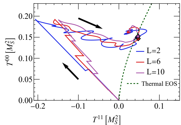
FIG. 10. Energy density versus pressure modelled with T^{00} and T^{11} , respectively, during the jet simulation. Three different subsystems with L = 2, 6, 10 are shown. We subtracted the vacuum values; hence, the curves start in the origin ( t = 0 ) moving initially to negative pressures before turning around and approaching the thermal equation of state (EOS). The diamonds indicate t_0 \approx 21.4/M_s . The arrows show the flow of time.
