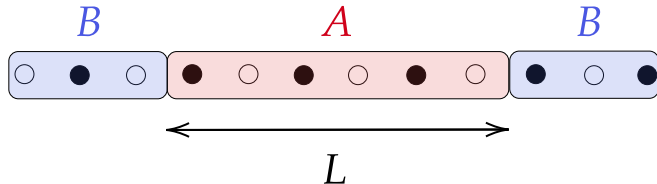
FIG. 5. The bipartition of the system used to study the entanglement of the central region of length L (subsystem A ) with the complement (subsystem B ). Subsystem A is centered around the center of the system.
