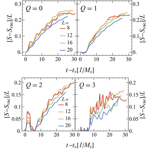
FIG. 18. Emergence of volume law in the time evolution of symmetry-resolved entanglement entropy in the charge sectors Q = 0, 1, 2, 3 . Vacuum values of EE are subtracted, the result is rescaled by the subsystem size and time is shifted as explained in the text describing Fig. 7. Q = 0, 1 sectors exhibit features similar to the full entanglement entropy, to which they provide dominant contributions (along with Q = -1 that is the same as Q = 1 ). In Q = 2 sector one can see that the volume law is approximately satisfied almost from the beginning. On the contrary, in Q = 3 sector we do not find volume law in small subsystems (which can be attributed to the fact that there are only a few states with Q = 3 in these subsystems).
