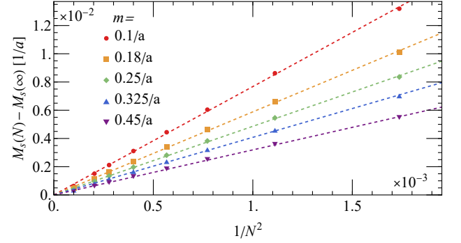
FIG. 16. Masses of the first excited states shown for a variety of fermion mass values m as functions of the inverse square of the system size N . Linear fits for infinite volume extrapolation are shown in dashed lines. Infinite volume extrapolated values are subtracted. Fermion coupling is g = 0.5/a .
