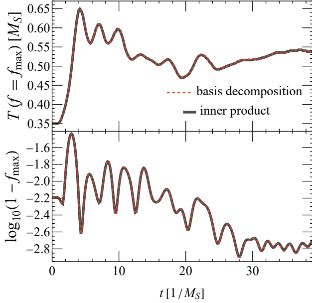
FIG. 21. Top panel: time dependence of temperature of the thermal state with maximal overlap with the reduced density matrix for a jet system describing subsystem of sites number 49 and 50. Bottom panel: the log of difference between the maximal overlap and 1. In both panels, the dashed red lines refer to the overlaps found from comparing local observables, as in Eq. (F4). The solid black lines refer to the overlaps found from Eq. (27) by taking inner products of MPOs, see the discussion in Section V of the main text. The two methods produce identical results, providing a cross-check of the validity of both.
