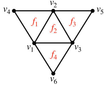
Figure 8: A part of a triangulated 2-manifold. Each face (2-simplex) is labeled with the red color.
