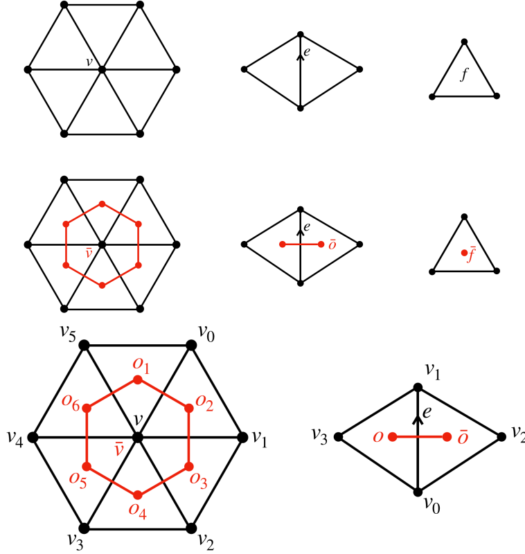
Figure 10: Dual cell complex in 2-d case.
