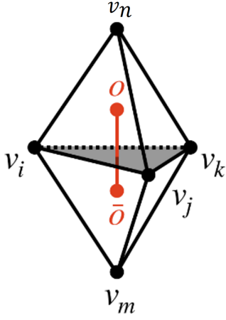
Figure 11: Example in 3-D.
