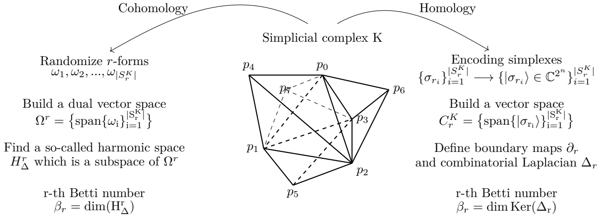
Figure 5: A diagram capturing the essential steps and main flow of quantum algorithms for estimating Betti numbers using the cohomology and homology frameworks, respectively.
