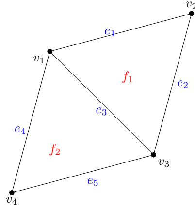
Figure 3: A part of a 2-D triangulated manifold, which contains two triangles (or 2-simplex) glued together. From a graph perspective, we have a set of vertices v_1, v_2, v_3, v_4 , edges (1-simplex) e_1, e_2, e_3, e_4 , and faces (2-simplex) f_1, f_2 . The above figure could be specified by some functions that describe the local connectivity between points/edges/faces as well as the inclusion relation between point-edge or edge-face.
