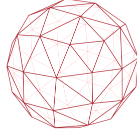
Figure 2: A triangulated sphere
