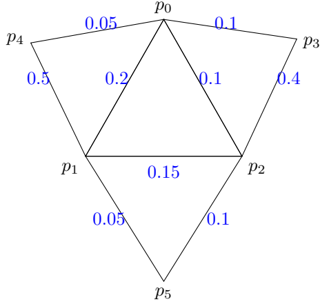
(a) Illustration of 1-form: \omega^1 essentially assigns each edge, or 1-simplex, to a real number
