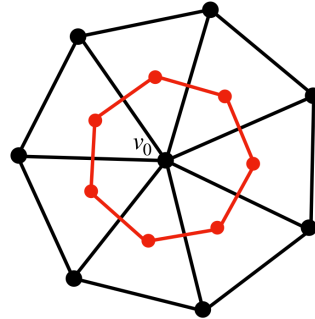
Figure 9: Illustration of dual cell of 0-simplex v_0 . The whole region inside the red-colored boundaries is the dual cell of v_0 , with area denoted as |v_0| . This area could be computed given the pairwise distance between v_0 and its adjacent vertices. In our case where the given triangulation is nearly uniform and the distance between two vertices is a , it is easy to calculate the area |v_0| , which is pa^2/4\sqrt{3} , where p is the number of adjacent points to v_0 .
