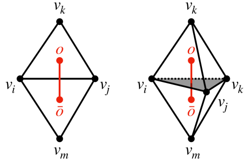
Figure 6: Dual cell complexes in 2 and 3 dimensions. Left figure: In a triangulated 2-manifold, the dual to 2-simplex [v_i, v_j, v_k] is a point o . The dual to an edge [v_i, v_j] is an edge o\bar{o} . Right figure: In a triangulated 3-manifold, the dual to 3-simplex [v_i, v_j, v_k, v_m] is a point o . The dual to a face (2-simplex) [v_i, v_j, v_k] is an edge o\bar{o} .
