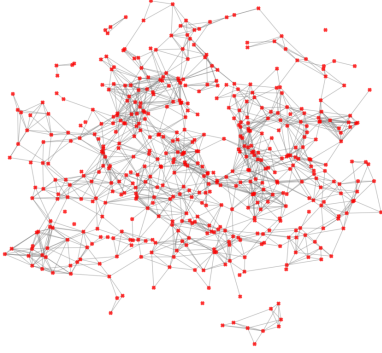
Figure 1: (a) Application of TDA in medical imaging: performing topological denoise. (b) An example of point cloud. Each point might be a vector in a very high dimension. Upon an appropriate metric, one can define distance between two points, and set a threshold for connectivity, e.g., two points are connected if their distance is less than some value. Roughly speaking, a point is called 0-simplex, an edge connecting two points is called 1-simplex, a triangle having 3 points mutually connected is called 2-simplex. Higher dimensional simplex is generalized in a straightforward manner. Then the resultant configuration forms a so-called simplicial complex. The goal of TDA is to analyze the underlying structure of given data points by using tools from algebraic topology, more concretely, homology theory.
