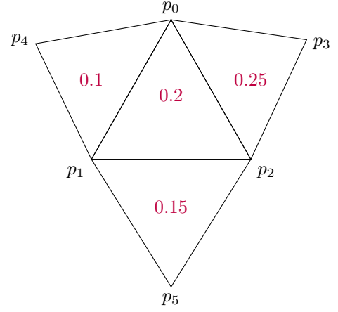
(b) Illustration of 2-form: \omega^2 essentially assigns each triangle, or 2-simplex, to a real number
