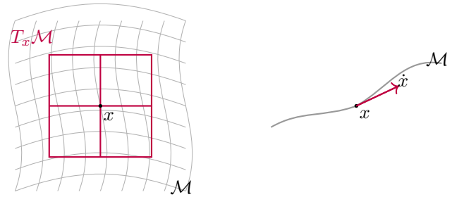
Figure 7: A tangent vector \mathcal{X}' is defined at a point \mathcal{X} \in \mathcal{M} . The collection of these tangent vectors forms a linear vector space at \mathcal{X} .
