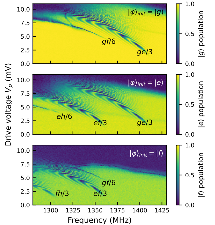
Figure 2. Parametric processes near one third of the qubit frequency. Multiple transitions can be activated by preparing initial states |g\rangle , |e\rangle , and |f\rangle and sweeping drive amplitude and frequency. The drive voltage V_p represents the peak amplitude of a pulse at the base stage of the dilution refrigerator.
