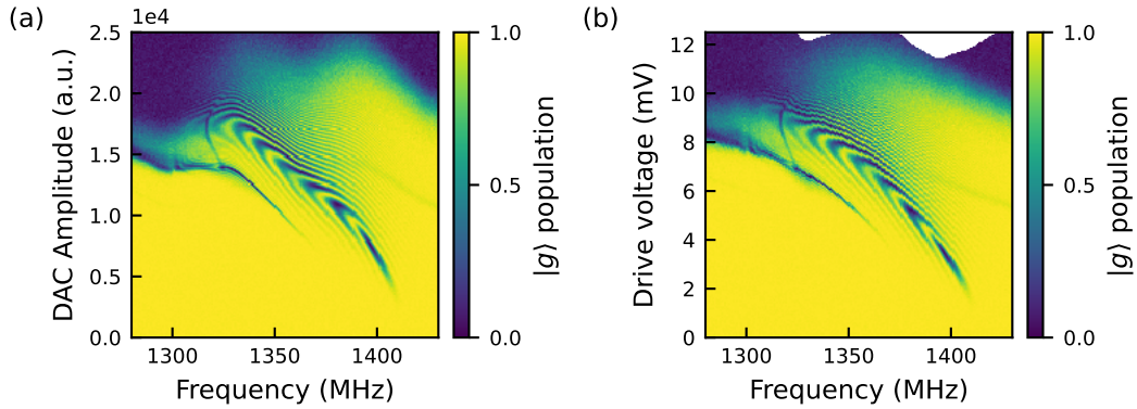
Figure S8. The power Rabi experiment (a) without amplitude correction and (b) with amplitude correction.
