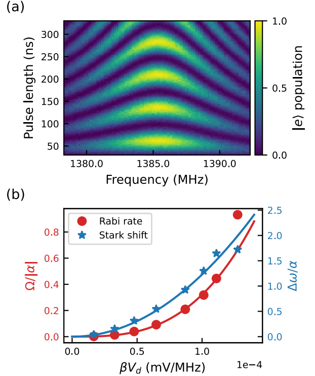
Figure 3. Rabi rate and ac-Stark shift vs. subharmonic driving strength. a A Rabi experiment for subharmonic driving of the qubit as a function of pulse duration and drive frequency at fixed drive amplitude of 4.71 mV. At this amplitude, the Rabi rate is 2\pi \times 13.55 MHz and the drive-induced qubit ac-Stark shift is 2\pi \times 81.25 MHz, equivalent to 0.55 times of the transmon anharmonicity \alpha . b Rabi rate and qubit ac-Stark shift vs. drive amplitude. The Rabi rate (red squares) is proportional to drive amplitude cubed. The ac-Stark shift (blue stars) is proportional to drive amplitude squared. A single fit function describes both sets of data with only one free parameter, the scaling factor k converting pulse amplitude \beta V_p to the effective driving strength \eta .
