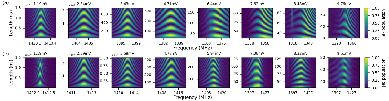
Figure S9. Subharmonic Rabi oscillations under different driving amplitudes with (a) the fixed frequency pulse and (b) the chirp modulated pulse.
