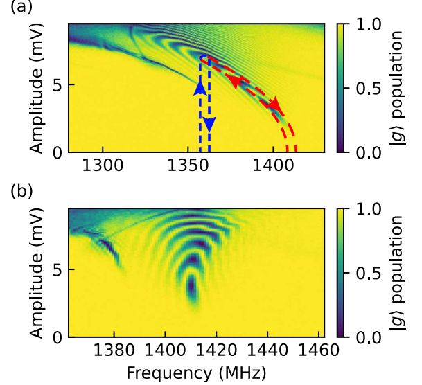
Figure 4. Amplitude-dependent frequency modulation of the drive frequency. a With the drive frequency following the ac-Stark shift of the transmon (red trace), a frequency chirped pulse is always resonant with the subharmonic process. Compared with fixed-frequency drive (blue trace), it avoids directly crossing other processes. b A power Rabi experiment with frequency chirping. The frequency axis here is the initial frequency of the pulse.
