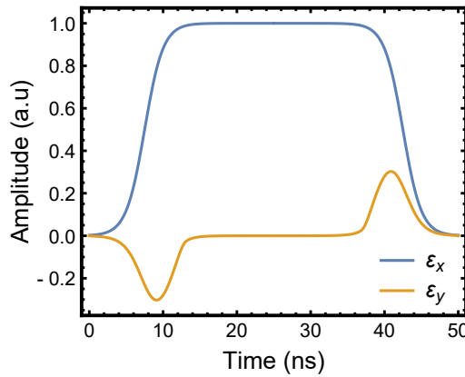
Figure S3. DRAG correction of a 50 ns flat-top pulse. The pulse with zero phase and without DRAG correction is defined to only have \varepsilon_x component, shown as the blue trace. The orange trace, \varepsilon_y component, is the DRAG correction of the pulse.
