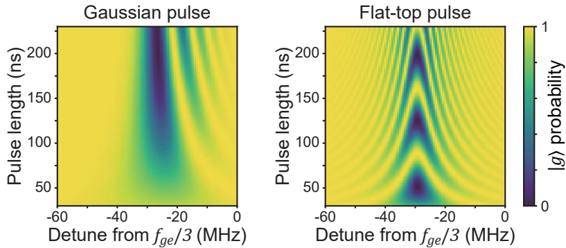
Figure S1. A simulation of fixed frequency Rabi experiment with the Gaussian pulse and the flat-top pulse.
