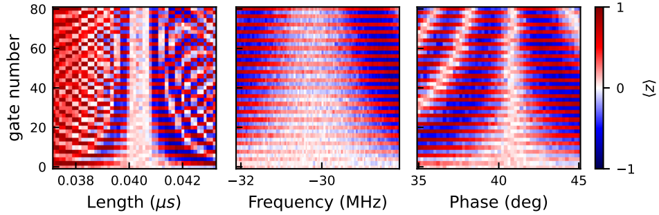
Figure S10. Fine tuning gate parameters. The transmon is prepared into the equator of the Bloch sphere with a \sqrt{X} gate, then followed by 2n \sqrt{X} gate, sweeping pulse parameters pulse length t_0 , modulating frequency \omega_{\text{mod}} and correcting phase. If the \sqrt{X} is well defined, \langle z \rangle should remain zero.
