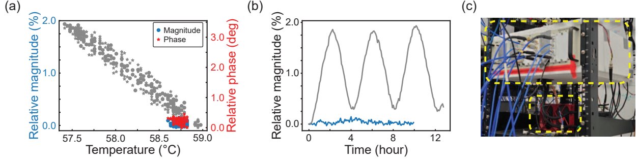
Figure S11. Temperature stability and its effect on pulse amplitude/phase. (a) The amplitude vs. temperature before (grey circles and stars) and after stabilization (blue circles and red stars). (b) The amplitude stability over time without stabilization (grey trace) and with stabilization (blue trace). The great improvement in pulse amplitude stability makes high fidelity control possible. (c) The experiment setup and a PID-controlled commercial liquid cooler are highlighted with yellow dashed boxes. The box is wrapped with Styrofoam except the front and back faces, which are for connecting coaxial cables. The liquid cooling head is mounted on the Al plate at the bottom of the box.
