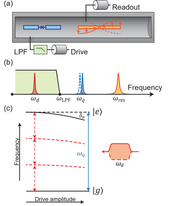
Figure 1. Subharmonic driving schematic. a A transmon qubit (at left in blue) and a \lambda/2 resonator for readout (at right in orange) are supported on a sapphire chip inside an aluminum tube. A low-pass filter (in green) is placed at the qubit drive port to suppress qubit photon leakage to the environment while allowing fast single qubit control at low frequencies. b The frequency distribution of the subharmonic drive \omega_d (red), qubit frequency \omega_{qe} (blue), and the readout resonator frequency \omega_{res} (orange). Only the subharmonic drive is within the pass-band of the LPF (green). The dashed, shifted peak of \omega_{qe} represents the ac-Stark effect during the subharmonic drive. c The energy level diagram of subharmonic driving. The ac-Stark effect induced by subharmonic drive creates a detuning \delta_p between the qubit's un-driven and driven frames. Flat-top pulses are used to control the qubit state.
