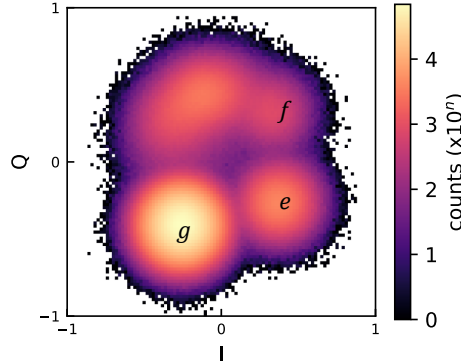
Figure S6. The histogram of transmon readout results.
