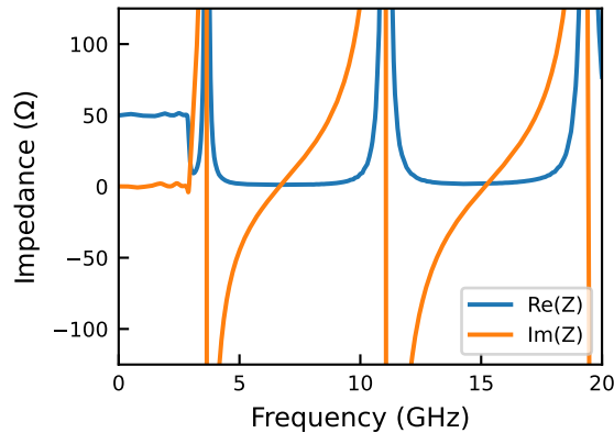
Figure S5. Impedance vs. frequency of low-pass filter used in the experiment
