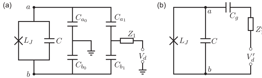
Figure S4. (a) The lumped-element circuit diagram of transmon with single drive port. (b) the reduced equivalent circuit.
