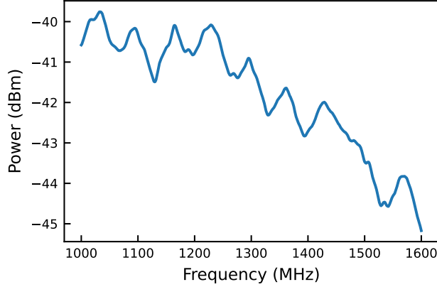
Figure S7. The microwave power at base stage vs. drive frequency.
