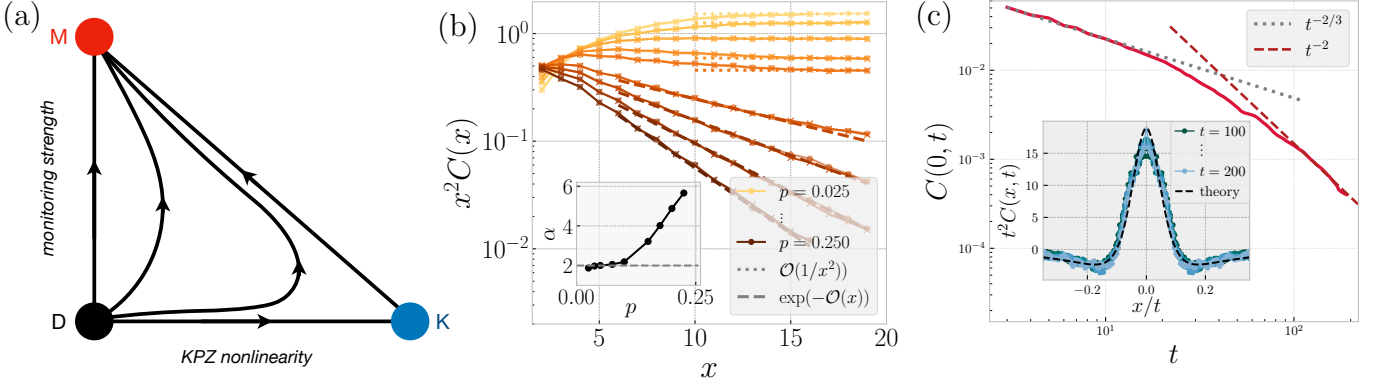
FIG. 3. Burgers' equation with weak monitoring. (a) The proposed renormalization-group flow shows the unstable fixed points D (diffusion) and K (KPZ), which flow to the stable free-boson fixed point M (monitored) at weak monitoring. For simplicity, we have not shown the strong monitoring phase and the KT-like phase transition here. We are also not depicting the full replica structure – the diagram depicts only the inter-replica degrees of freedom, the replica symmetric degrees of freedom are un-modified by monitoring. (b) The connected equal-time density-density correlator C(x) \equiv \mathbb{E}_{\mathbf{m}} [\langle \rho_x \rho_0 \rangle_{\mathbf{m}} - \langle \rho_x \rangle_{\mathbf{m}} \langle \rho_0 \rangle_{\mathbf{m}}] (conditional on a typical measurement, i.e., drawn according to its likelihood) as a function of distance: consistent with the field theory prediction, this correlation function follows a power-law with exponent \alpha = 2\Delta_\rho close to 2 for weak measurement rate p (main and inset), while for stronger measurements the system enters the sharp phase and these correlations decay exponentially (main). The numerical data are on systems of size L = 80 and averaged over N \approx 1000 samples (measurement trajectories) [94]. For each measurement trajectory, the probability state vector is evolved using matrix product state methods with two different maximum bond dimension cutoffs \chi = 200, 300 , shown with circle ( \bullet ) and cross ( \times ) markers, to verify convergence. The values of the measurement rate for the various curves are p \in \{0.025, 0.0375, 0.05, 0.075, 0.1, 0.15, 0.175, 0.2, 0.225\} (light to dark). (c) Dynamical two-point function C(x, t) for TASEP under weak monitoring ( p = 0.025 ). The autocorrelator C(0, t) shows a clear crossover from the KPZ scaling C(0, t) \sim t^{-2/3} at early times to the predicted C(0, t) \sim t^{-2} decay at late times (main), consistent with flow to the stable monitored free-boson fixed point. Furthermore, we observe a scaling collapse of the full dynamical correlation function C(x, t) when plotted as a function of x/t (inset), consistent with the z = 1 scaling of the free-boson fixed point and showing qualitative agreement with the universal scaling function of Eq. (21). These simulations sample posteriors for typical measurement histories using a time-evolving block decimation (TEBD) algorithm with measurement rate p = 0.025 , system size L = 140 , and bond dimension \chi = 150 .
