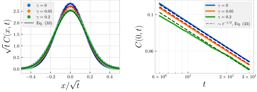
FIG. 2. Linear diffusion with gradient monitoring. (Left) The rescaled dynamical correlator \sqrt{t}C(x,t) plotted as a function of x/\sqrt{t} for monitoring strengths \gamma = 0, 0.05, 0.2 in the monitored noisy linear diffusive system described in Sec. IV B. Consistent with the field-theory prediction Eq. (33), the correlators collapse onto a Gaussian diffusive scaling form, with monitoring increasing the effective diffusion constant and therefore broadening the profile. The solid lines show the theoretical scaling function. (Right) The autocorrelator C(0,t) for the same values of \gamma , shown on a log-log scale. In all cases the decay follows the diffusive form C(0,t) \sim t^{-1/2} , with a \gamma -dependent prefactor D_{\text{eff}} = \sqrt{D^2 + c\gamma\sigma^2} with c \approx 1.4 , consistent with the renormalized diffusivity in Eq. (33). Numerical data is obtained using the Doob-tilted two-replica stochastic evolution described in Appendix VII.
