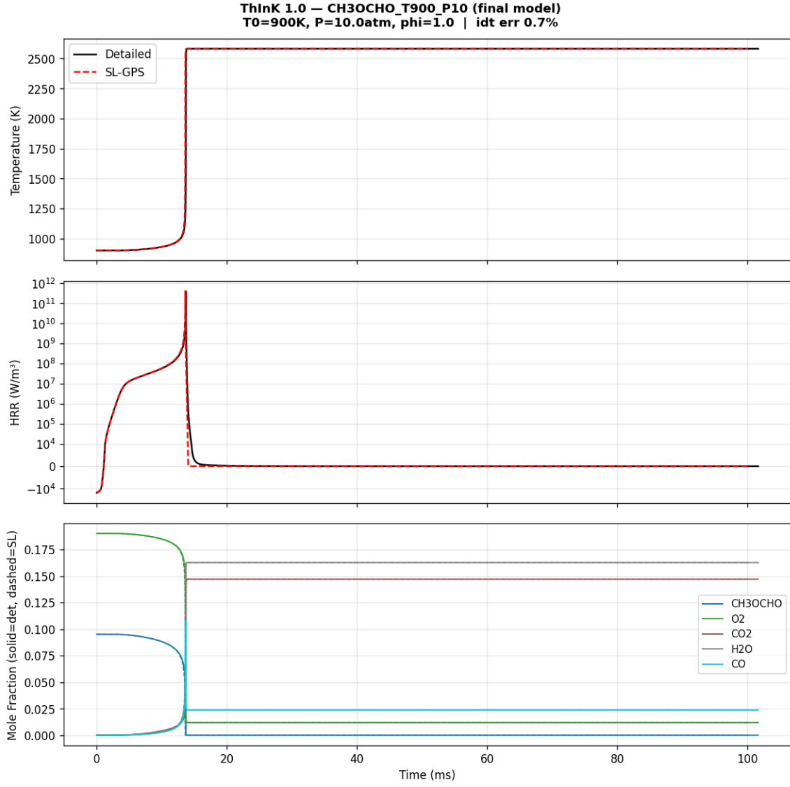
Figure 10: Final model, T900_P10 ( T_0 = 900 K, P = 10 atm, \phi = 1.0 ): the baseline failure (165.2%, Figure 6) is resolved — ignition delay error 0.7%.
