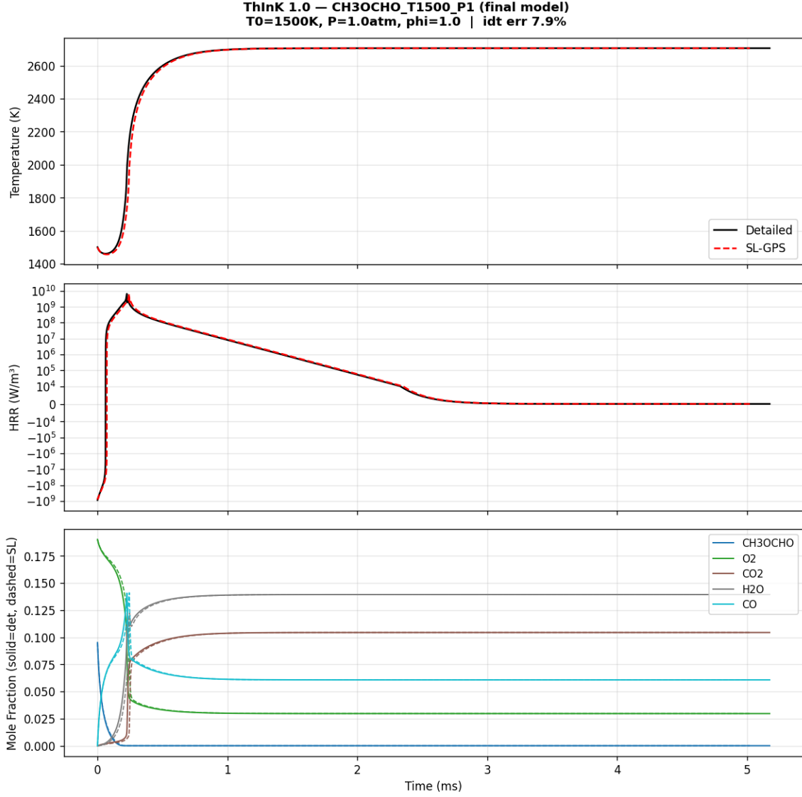
Figure 12: Final model, high-temperature case T1500_P1 ( T_0 = 1500 K, P = 1 atm): the Revision-2 regression (146.7%) is recovered to 7.9% error.
