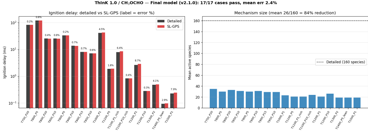
(b) Final model (v2.1.0, Revision 2): 17/17 cases, mean error 2.4%, 84% mean reduction.
