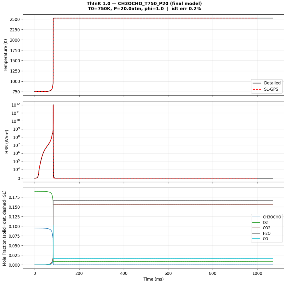
Figure 11: Final model, deep-NTC case T750_P20 ( T_0 = 750 K, P = 20 atm): two-stage ignition reproduced with 0.2% error.
