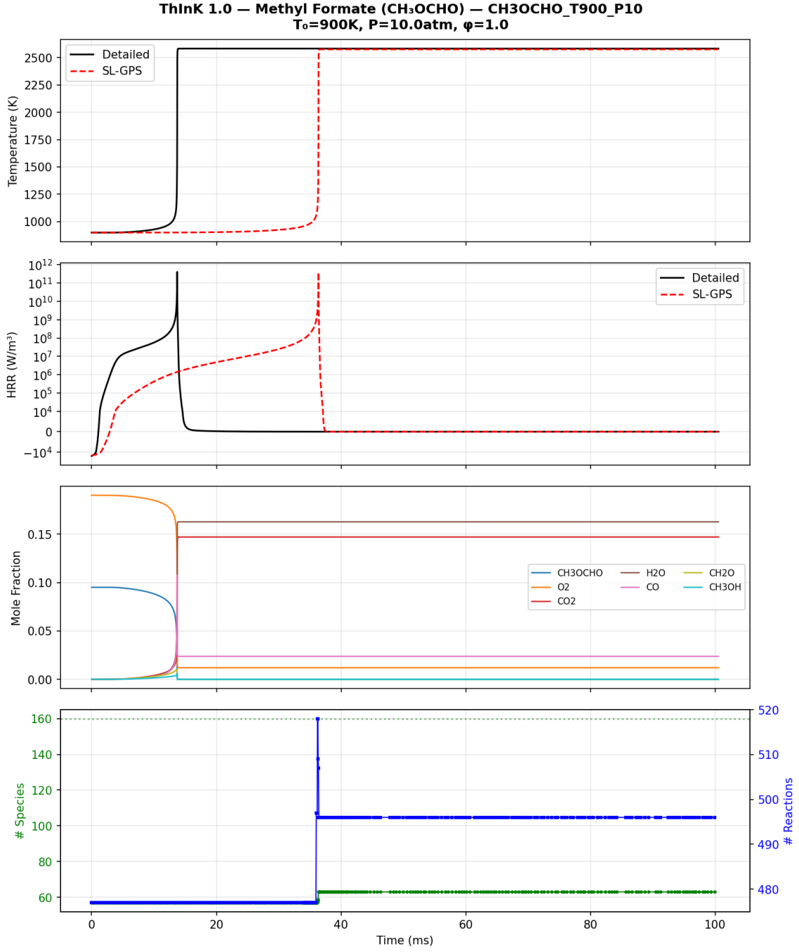
Figure 6: CH 3 OCHO Case 6 ( baseline model, before fixes ): T_0 = 900 K, P = 10 atm, \phi = 1.0 . Ignition delay error: 165.2%. This historical failure motivated the Revision 2 investigation and is resolved by the final model (0.7% error, Figure 10).
