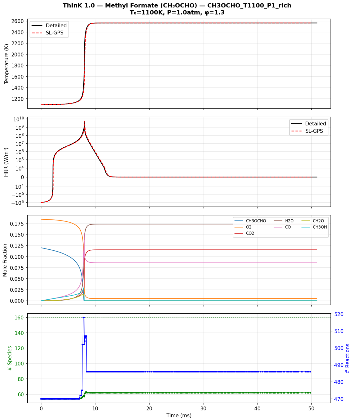
Figure 7: CH 3 OCHO Case 7: T_0 = 1100 K, P = 1 atm, \phi = 1.3 . Fuel-rich. Ignition delay error: 1.3%.
