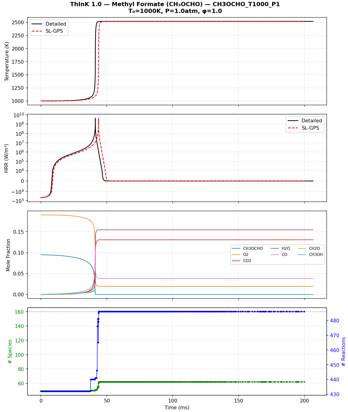
Figure 1: CH 3 OCHO Case 1: T_0 = 1000 K, P = 1 atm, \phi = 1.0 . Ignition delay error: 6.0%.
