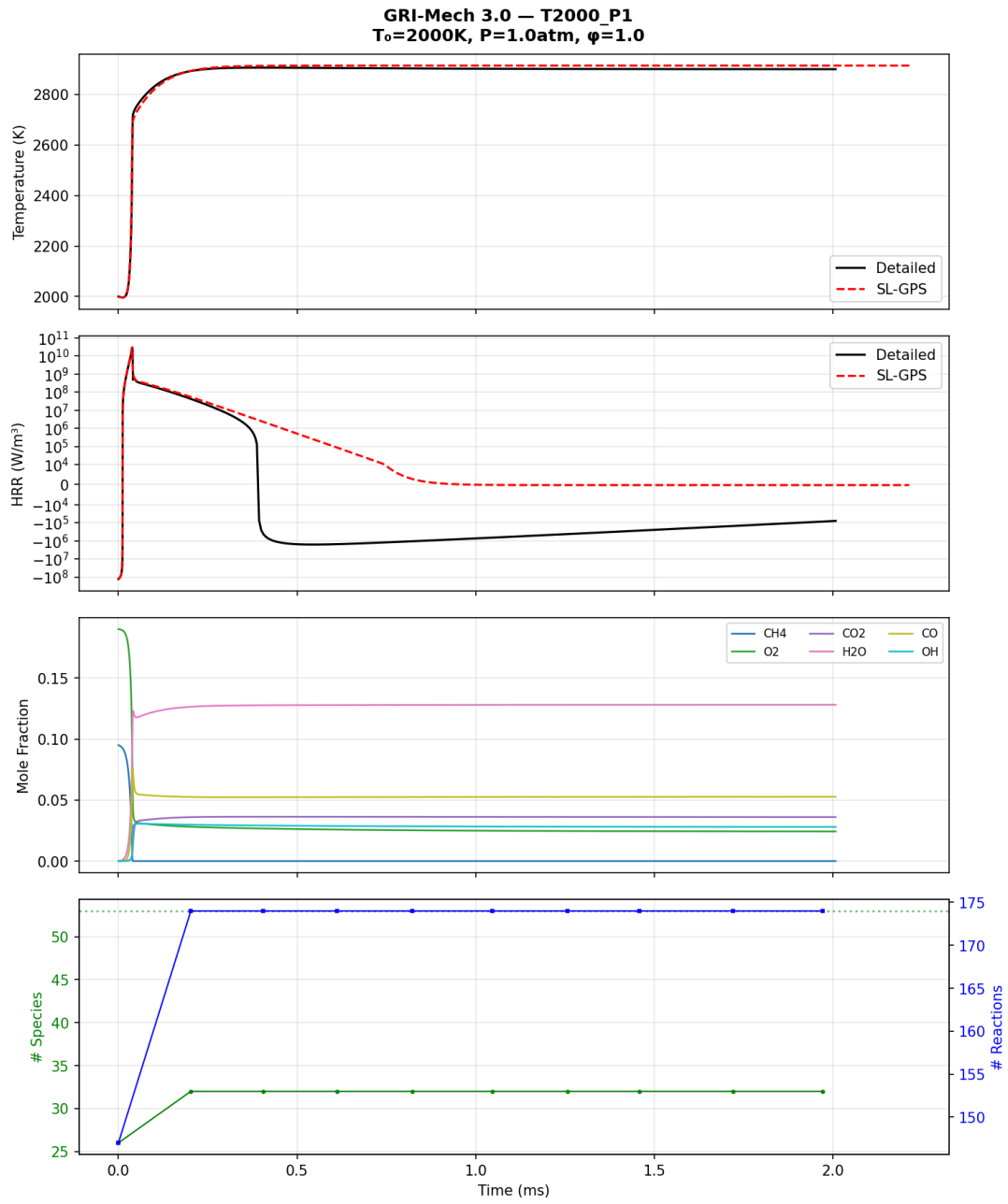
Figure 5: Case: T=2000K, P=1atm, \phi =1.0
