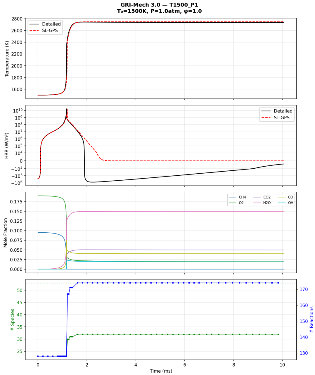
Figure 3: Case: T=1500\text{K} , P=1\text{atm} , \phi=1.0
