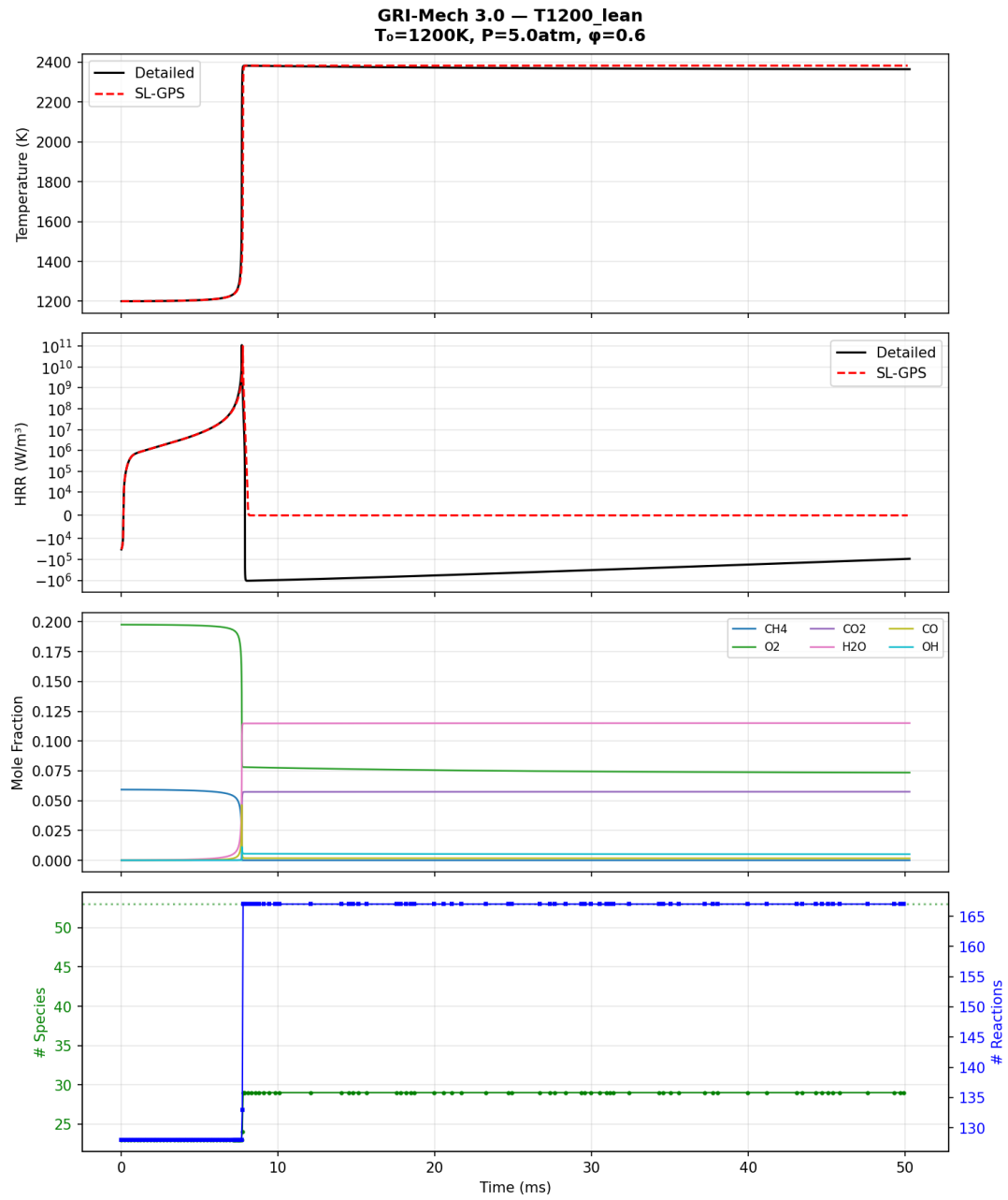
Figure 6: Case: T=1200\text{K} , P=5\text{atm} , \phi=0.6 (lean)
