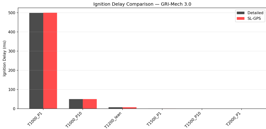
Figure 1: Ignition delay comparison: Detailed vs SL-GPS
