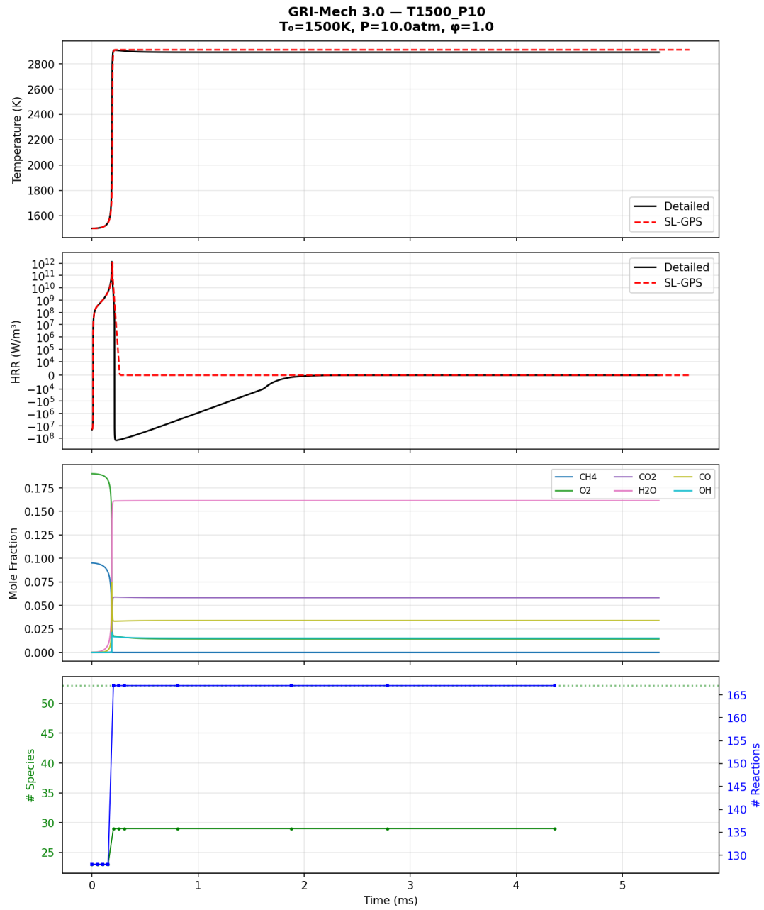
Figure 4: Case: T=1500K, P=10atm, \phi =1.0
