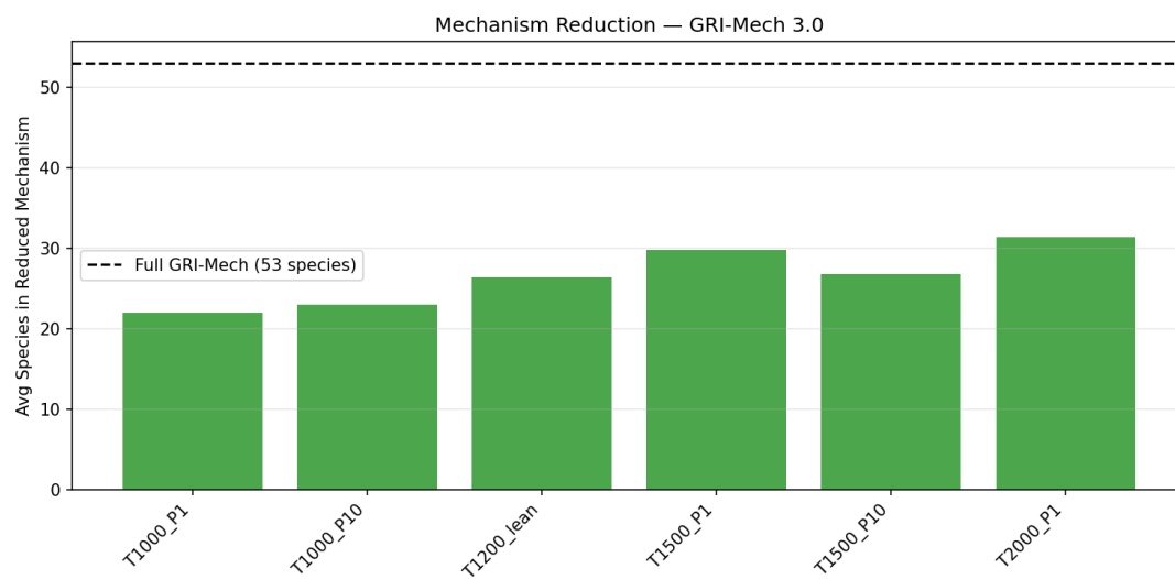
Figure 2: Average species count in reduced mechanism per case
