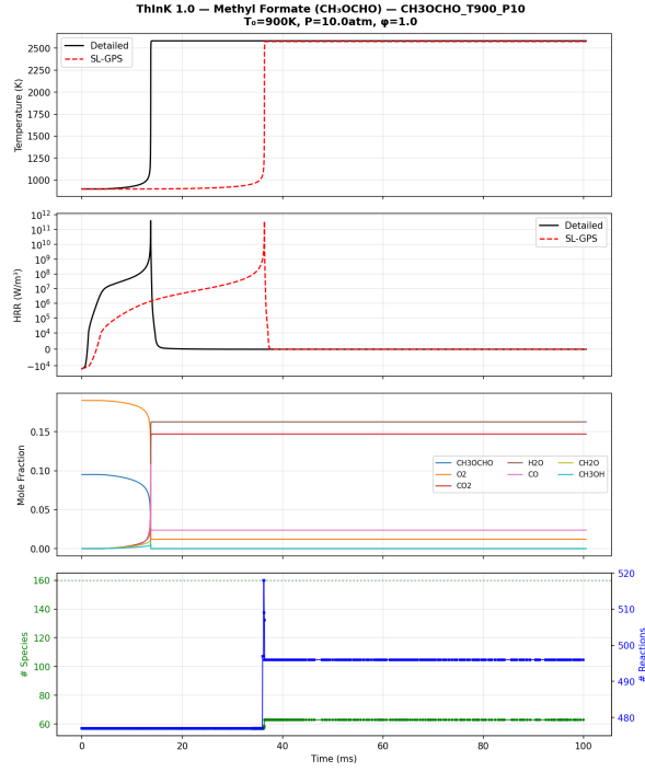
(a) Baseline model (before fixes): 165.2% error.
