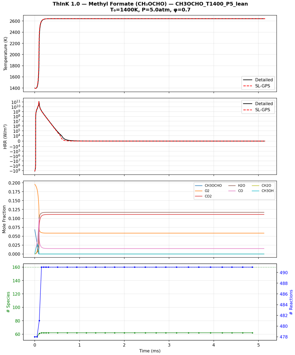
Figure 8: CH 3 OCHO Case 8: T_0 = 1400 K, P = 5 atm, \phi = 0.7 . Fuel-lean. Ignition delay error: 4.5%.
