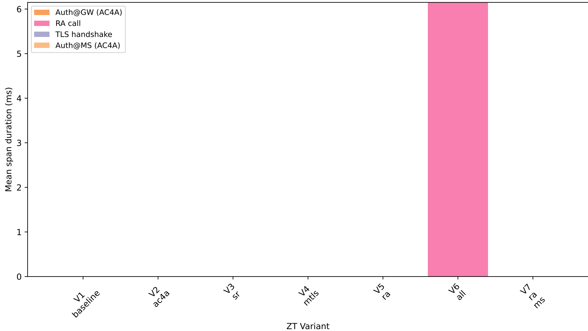
ZT Primitive Overhead Breakdown by Variant (HTTP pattern)
