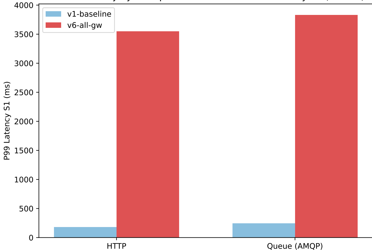
P99 S1 Latency by Transport — Baseline vs Full Gateway ZT (30 RPS)
