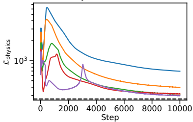
Physics Loss (multi)
