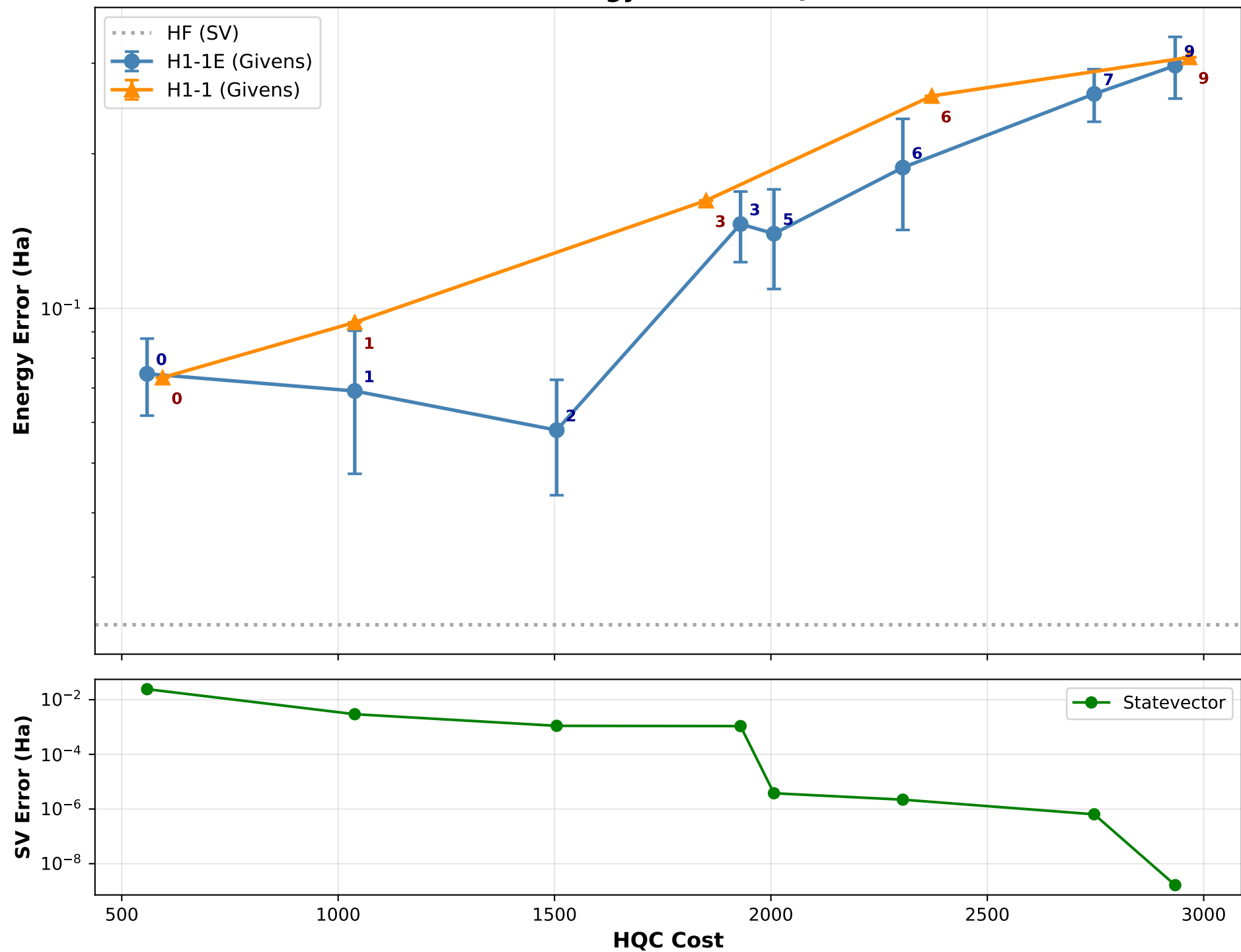
BeH2 - Energy Error vs HQC Cost
