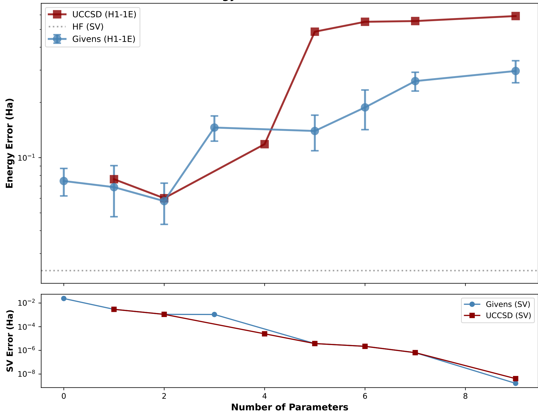
BeH2 - Energy Error vs Number of Parameters
