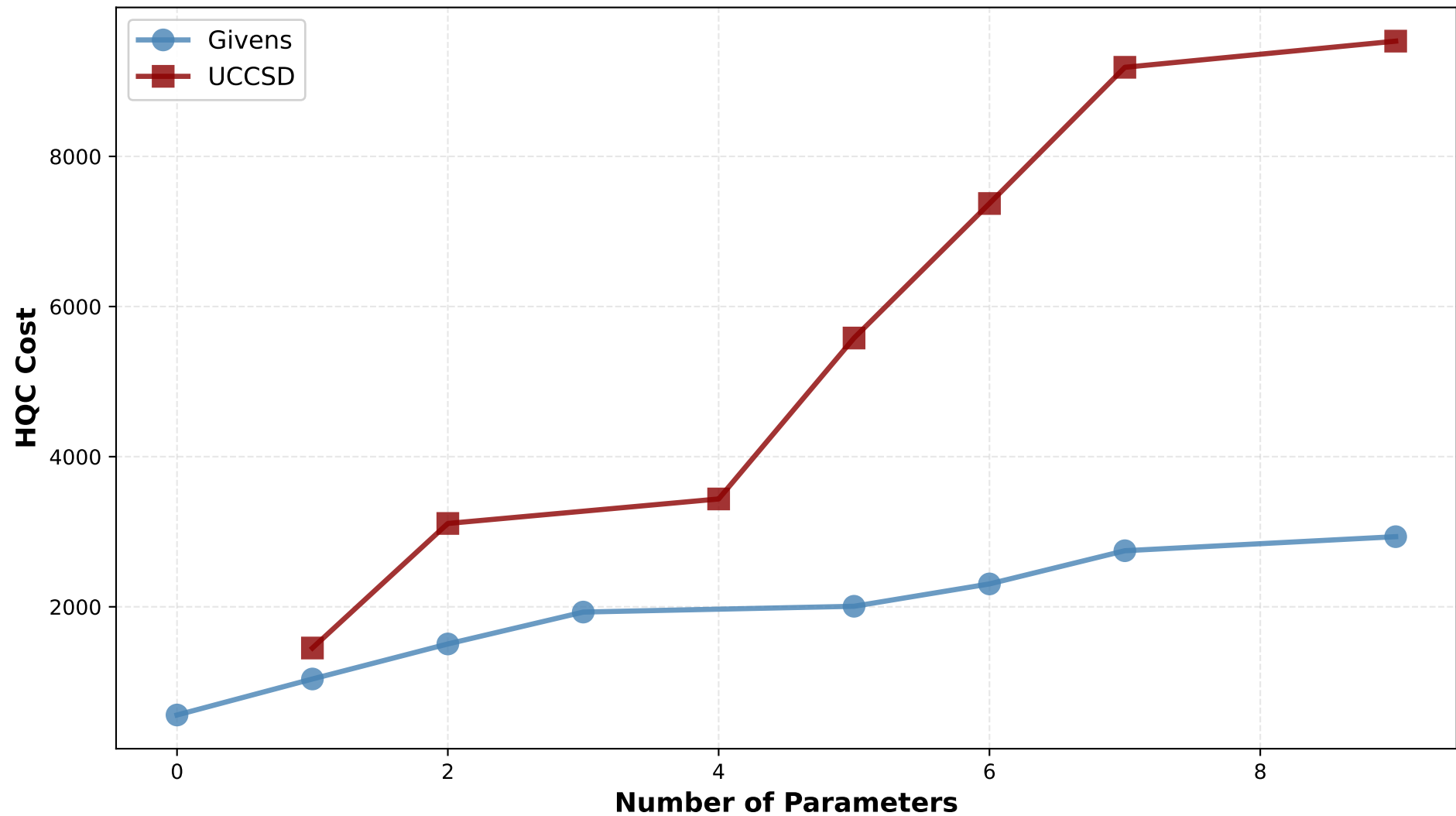
BeH2 - HQC Cost vs Number of Parameters (H1-1E)
