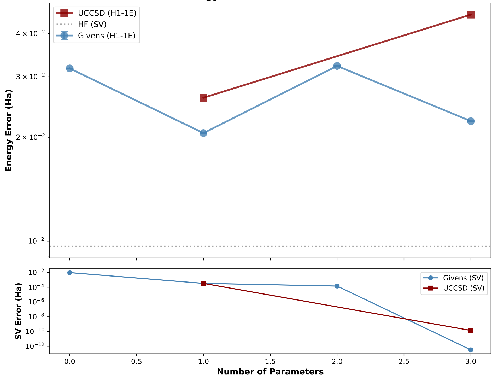
HeH - Energy Error vs Number of Parameters
