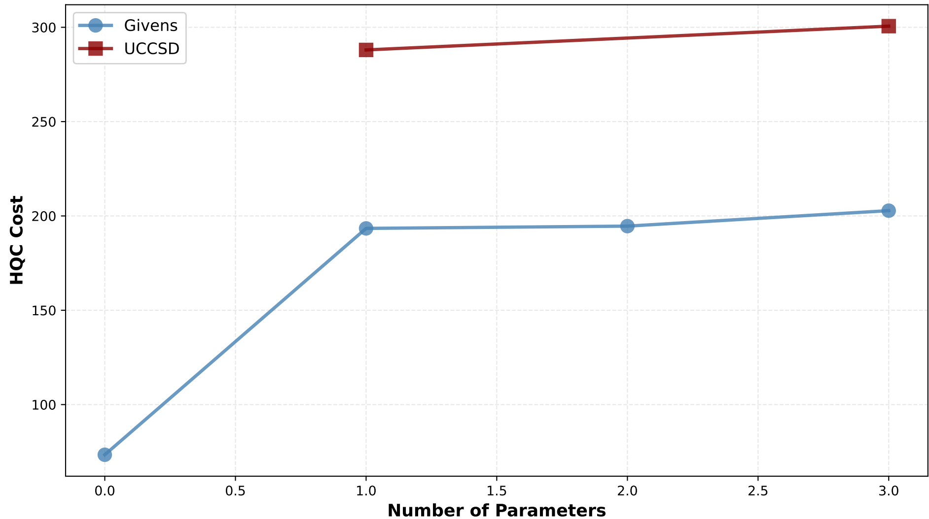
HeH - HQC Cost vs Number of Parameters (H1-1E)
